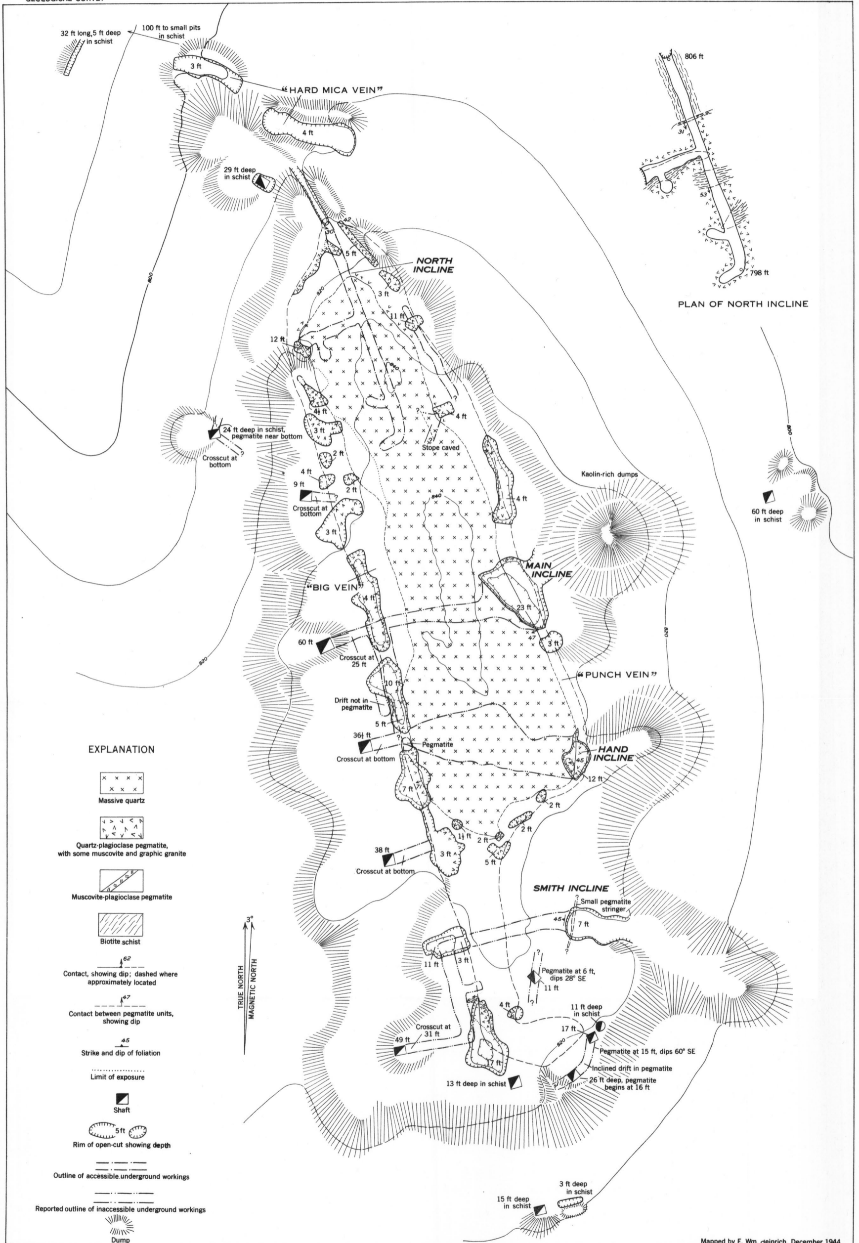
GEOLOGIC MAP AND PLAN OF THE MICA HILL MINE, TALLAPOOSA COUNTY, ALABAMA
