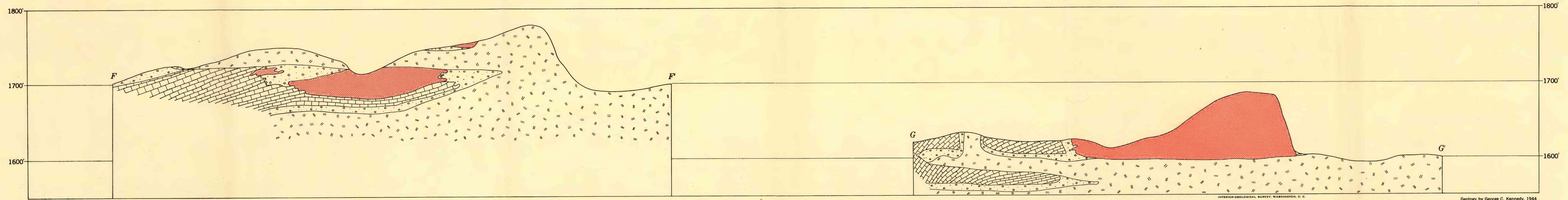
GEOLOGIC SECTIONS OF MAGNETITE CLIFF BODY, JUMBO BASIN, PRINCE OF WALES ISLAND, SOUTHEASTERN ALASKA
