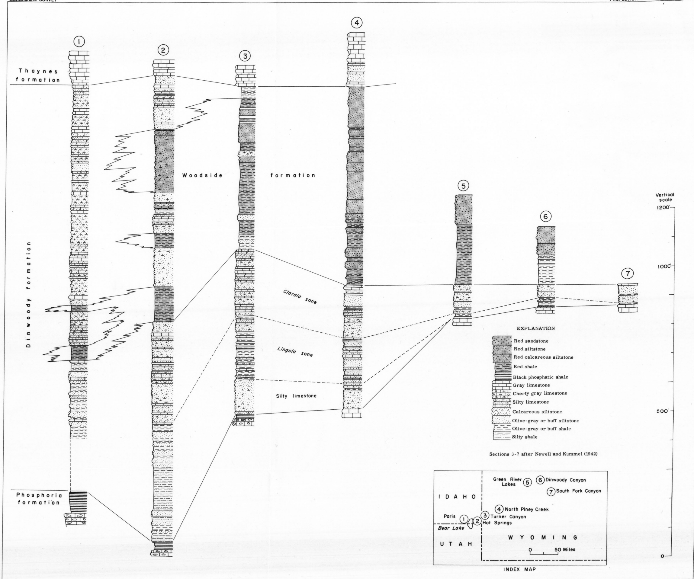
CORRELATION OF THE DINWOODY AND WOODSIDE FORMATIONS BETWEEN PARIS, IDAHO, AND THE WIND RIVER MOUNTAINS, WYOMING
