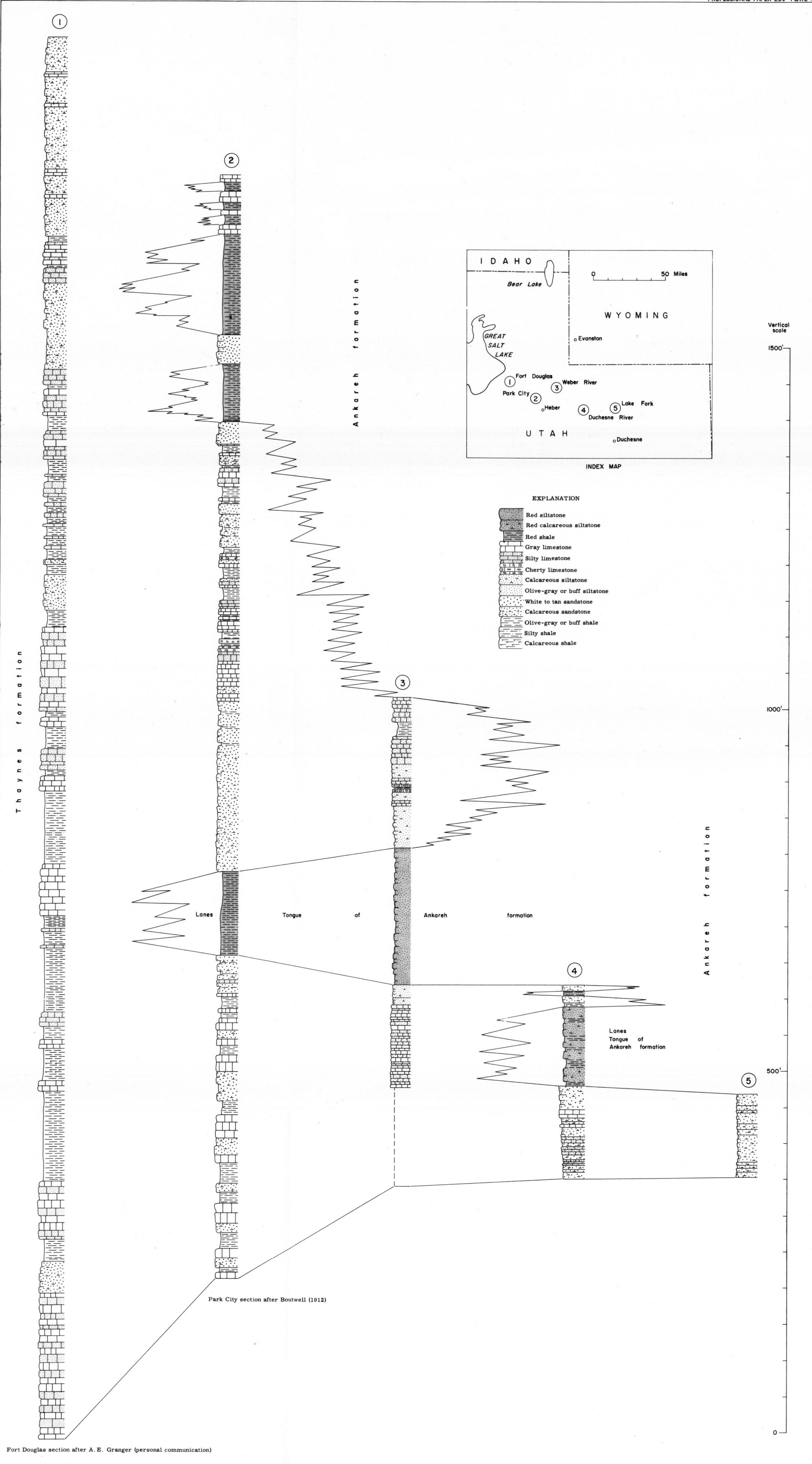
CORRELATION OF OUTCROP SECTIONS OF THE THAYNES FORMATIONS IN THE CENTRAL WASATCH AND UINTA MOUNTAINS, UTAH
