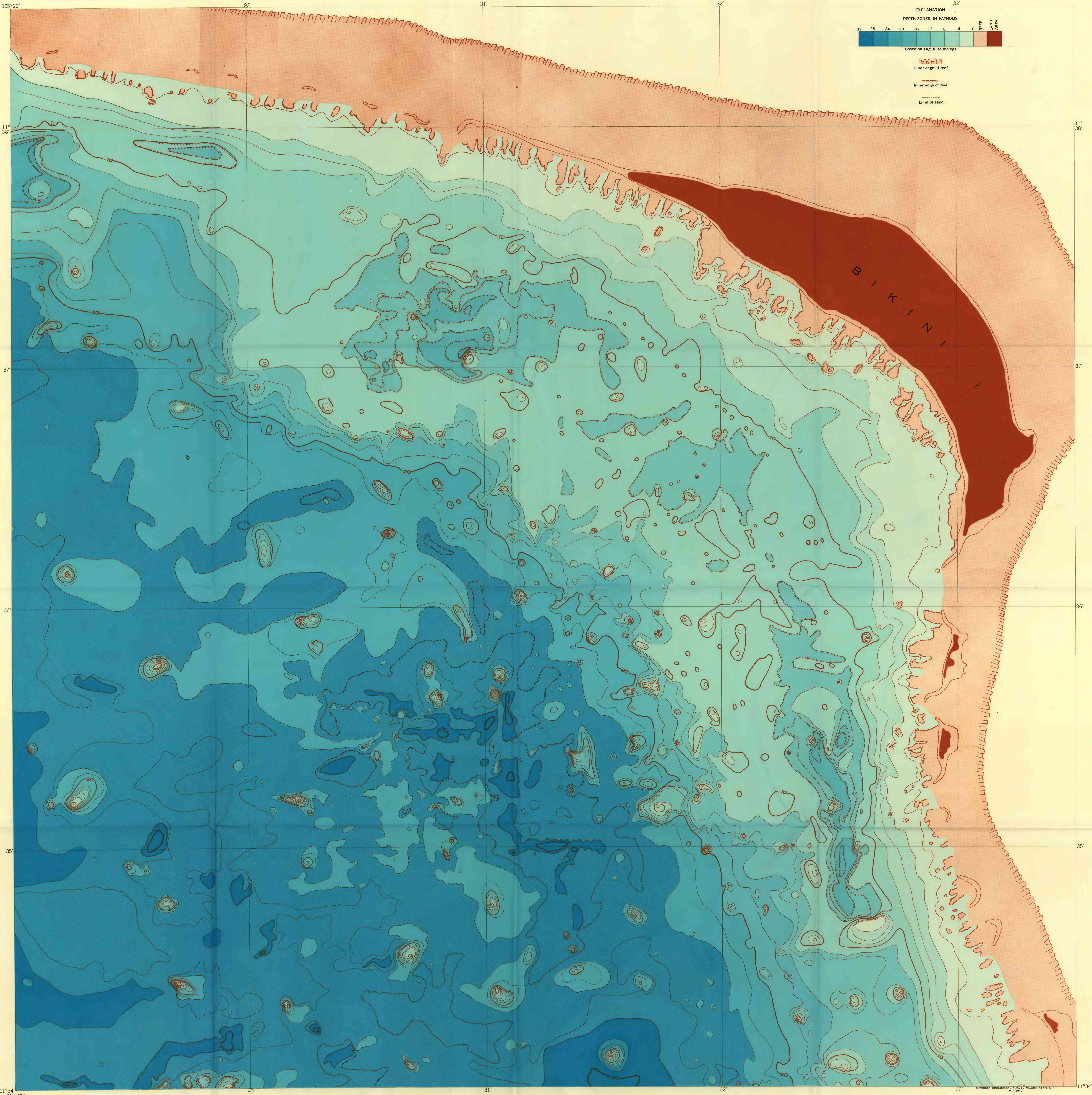
DETAILED CONTOUR CHART OF NORTHEASTERN CORNER OF BIKINI LAGOON
