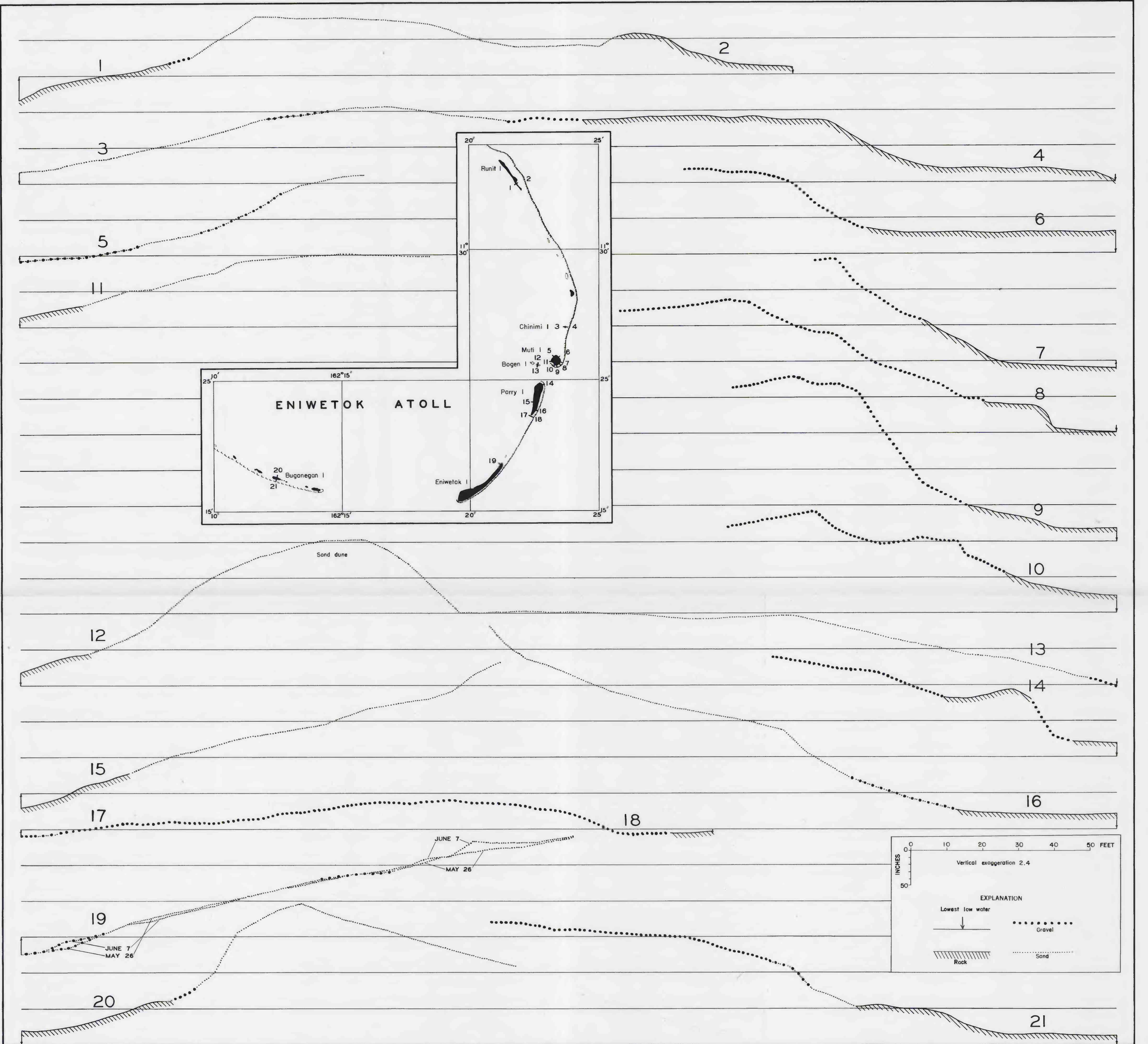
BEACH PROFILES AT ENIWETOK ATOLL
