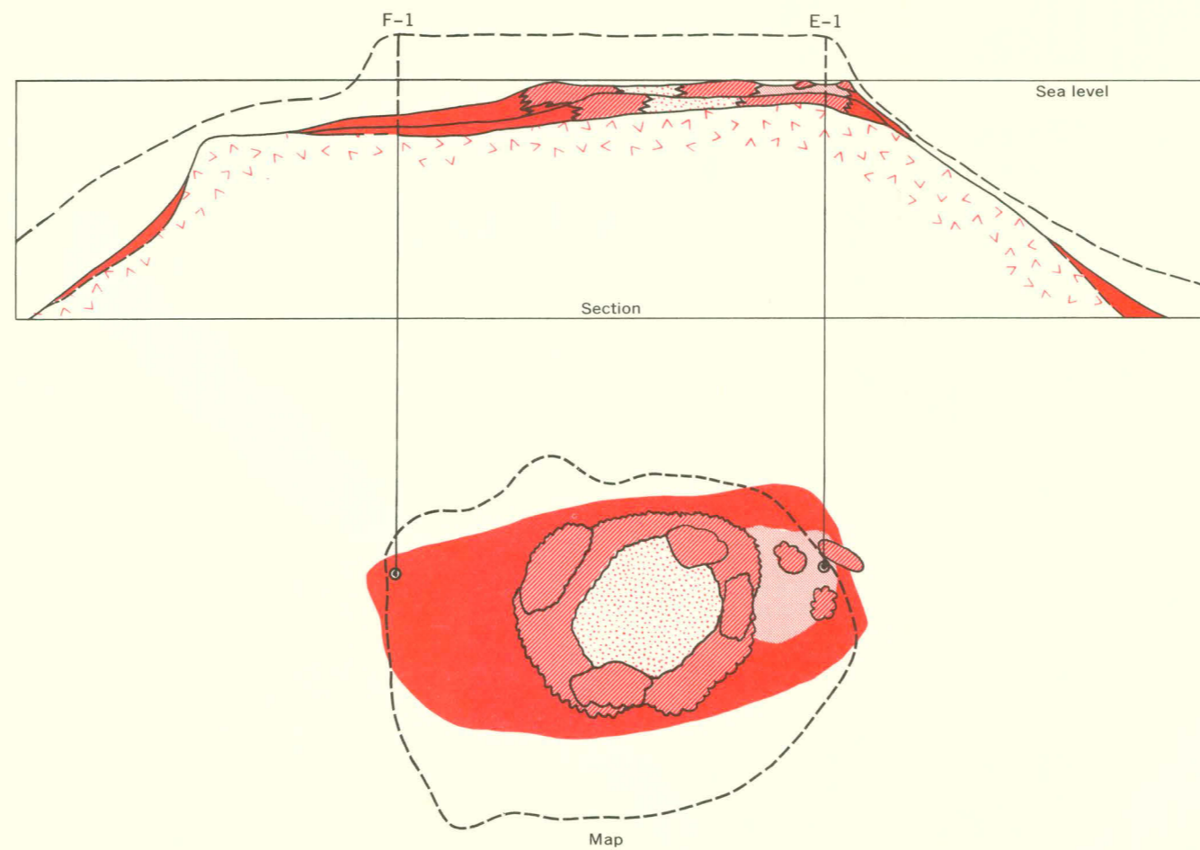
B. During Peneroplis-Triloculina time; Tertiary b
