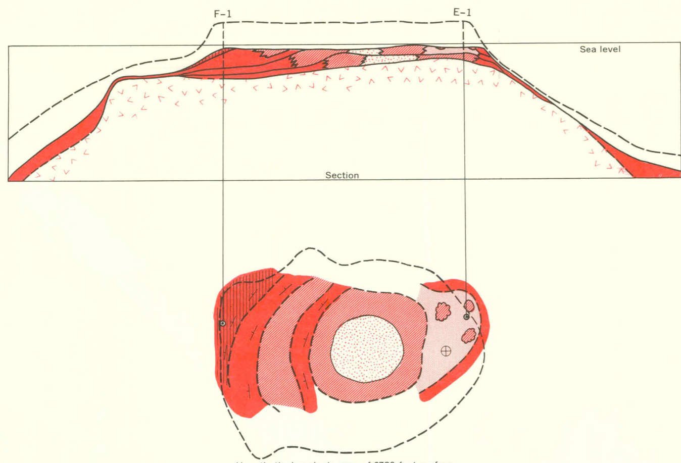
Hypothetical geologic map of 2780-foot surface D. Following truncation at 2780 feet; Tertiary e
