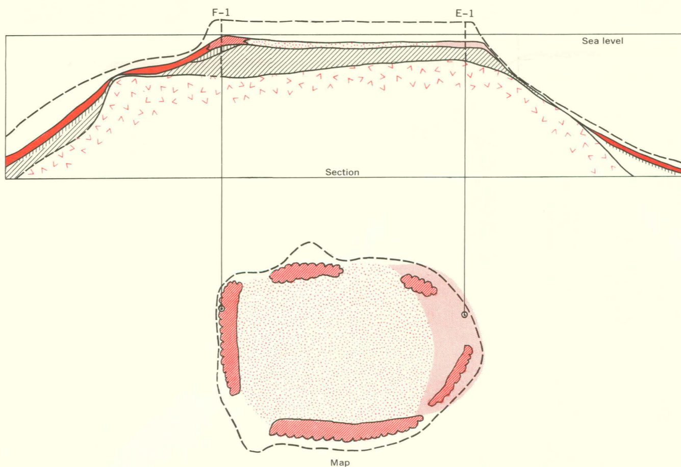
E. During deposition of Lithophyllum zone; Tertiary e
