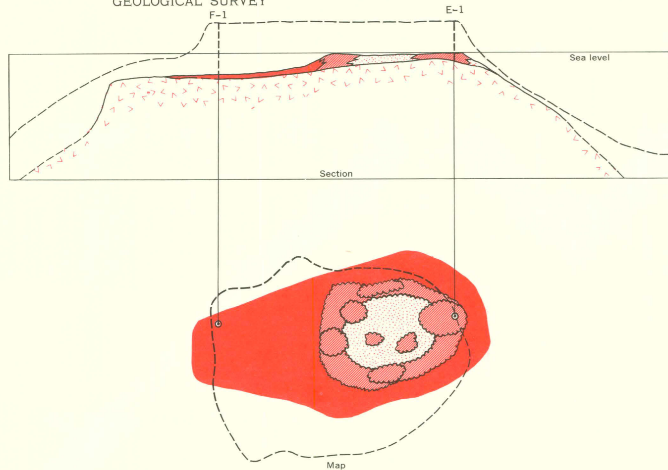
A. In pre- Asterigerina rotula time; Tertiary b
