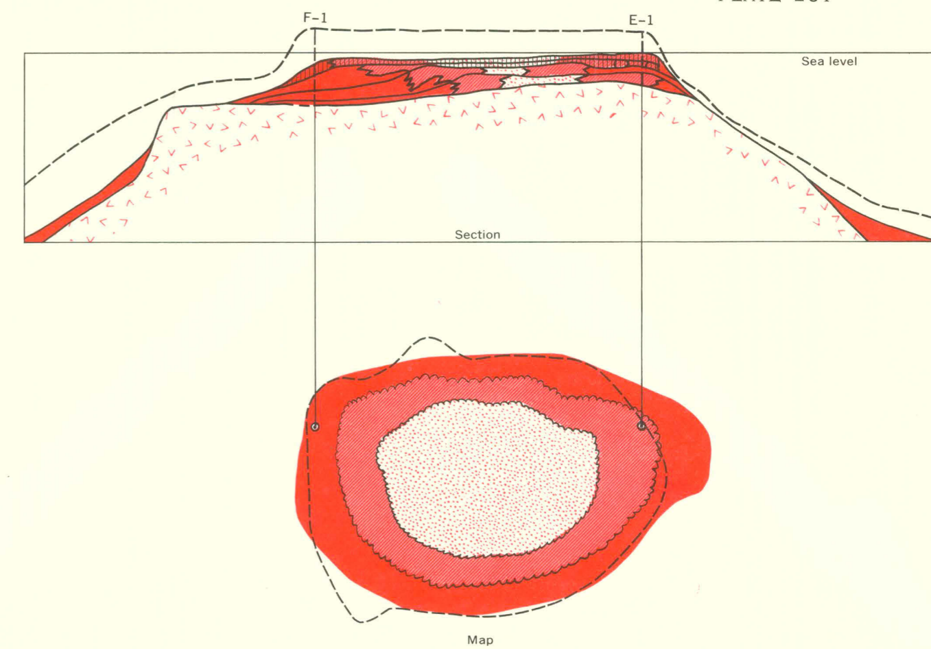
C. In early Tertiary e time
