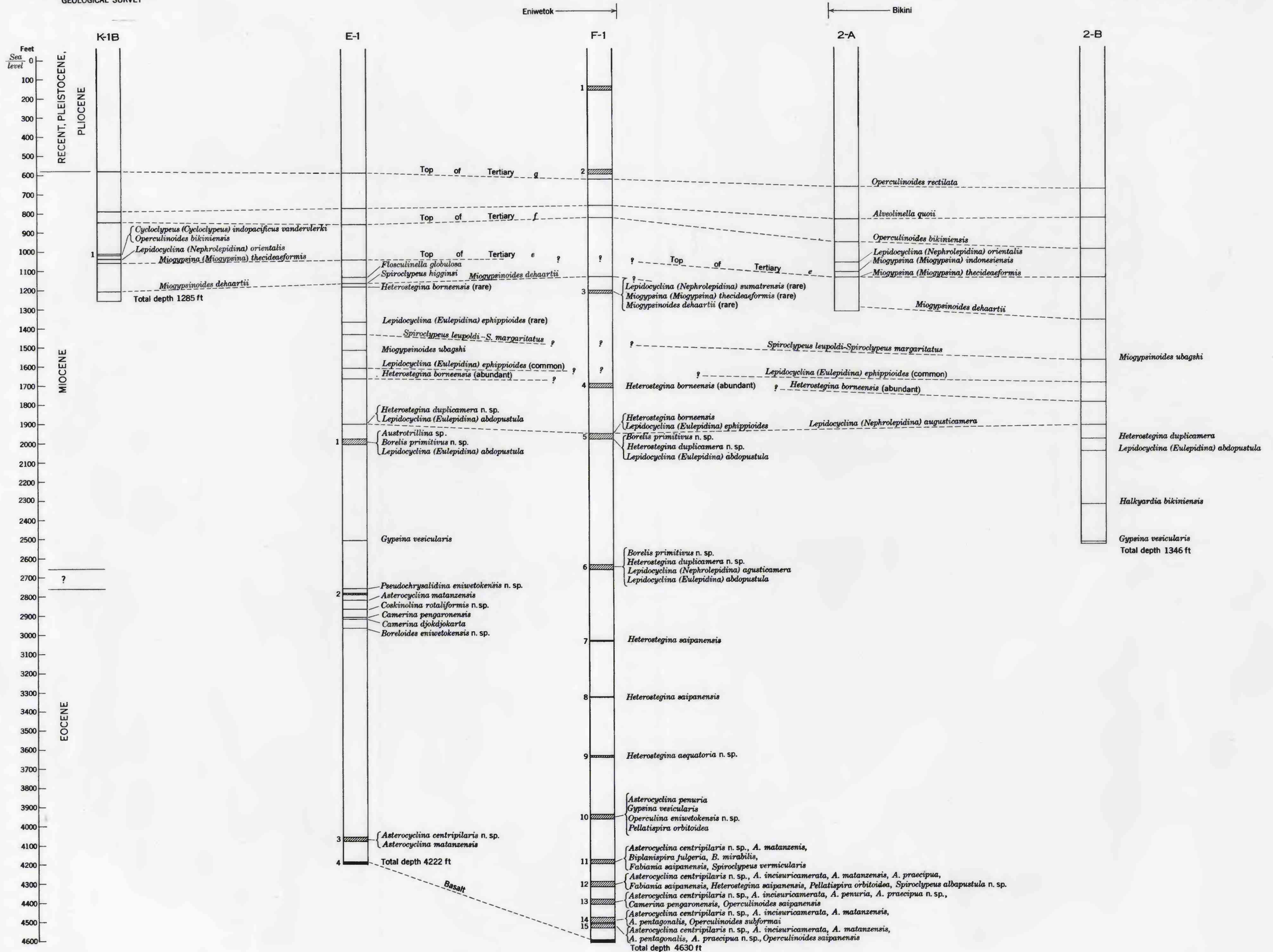
CORRELATION OF THE ENIWETOK ATOLL AND BIKINI ISLAND DRILL HOLES
