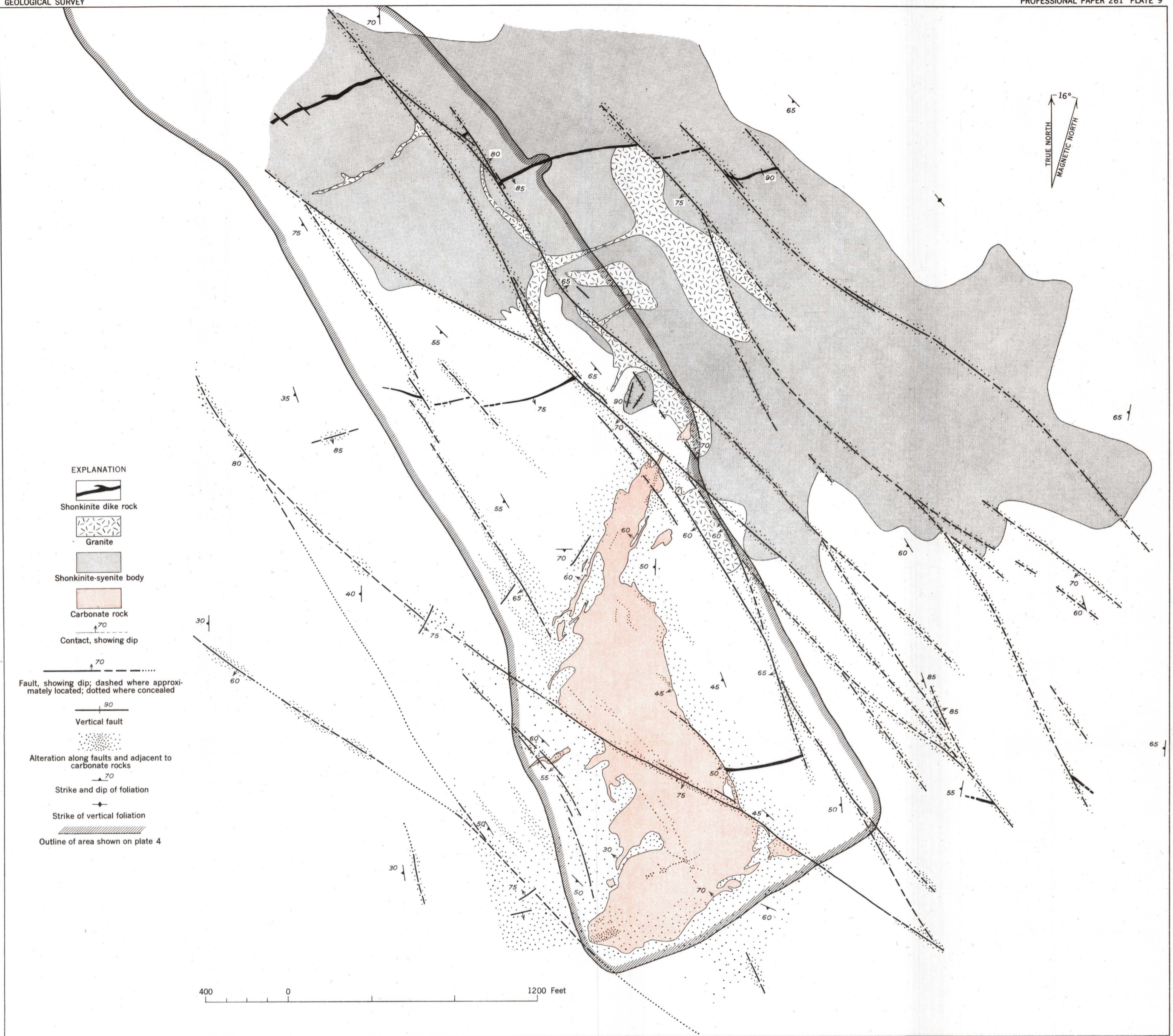
MAP SHOWING MAJOR STRUCTURAL FEATURES IN VICINITY OF SULPHIDE QUEEN CARBONATE BODY, MOUNTAIN PASS DISTRICT, CALIFORNIA
