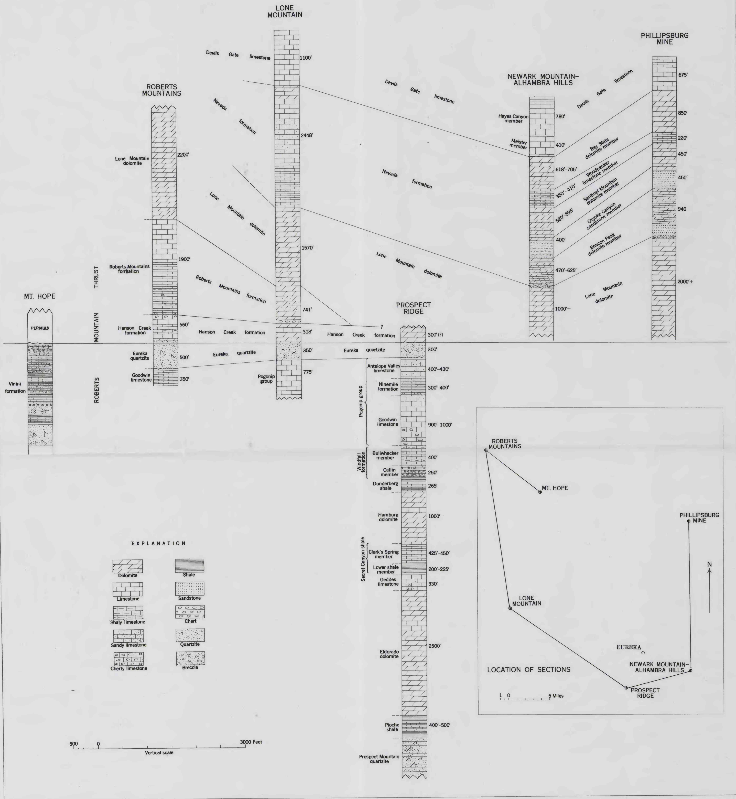
STRATIGRAPHIC SECTIONS OF LOWER AND MIDDLE PALEOZOIC ROCKS IN THE VICINITY OF EUREKA, NEVADA
