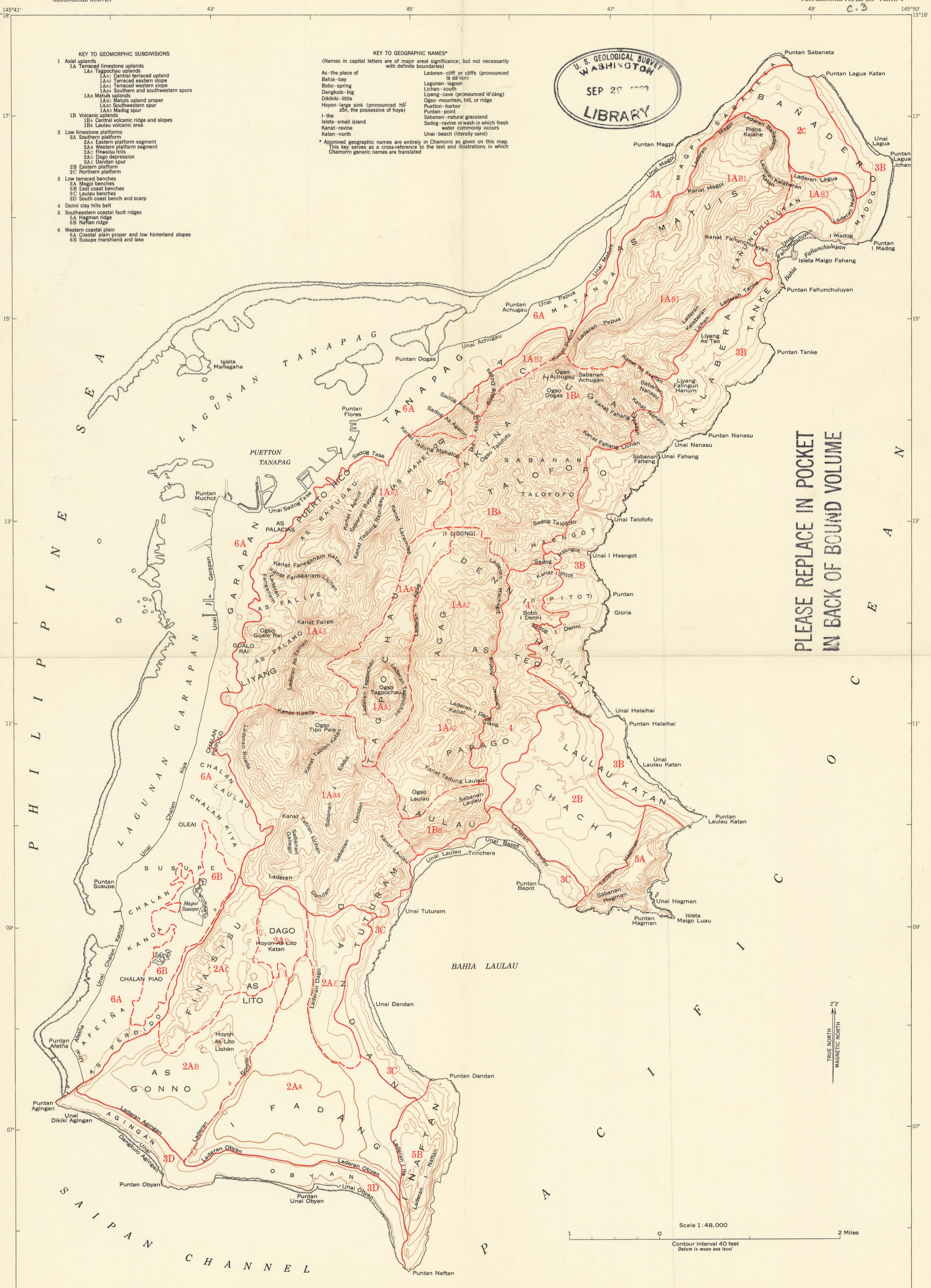
TOPOGRAPHIC AND GEOMORPHIC MAP OF SAIPAN, MARIANA ISLANDS
