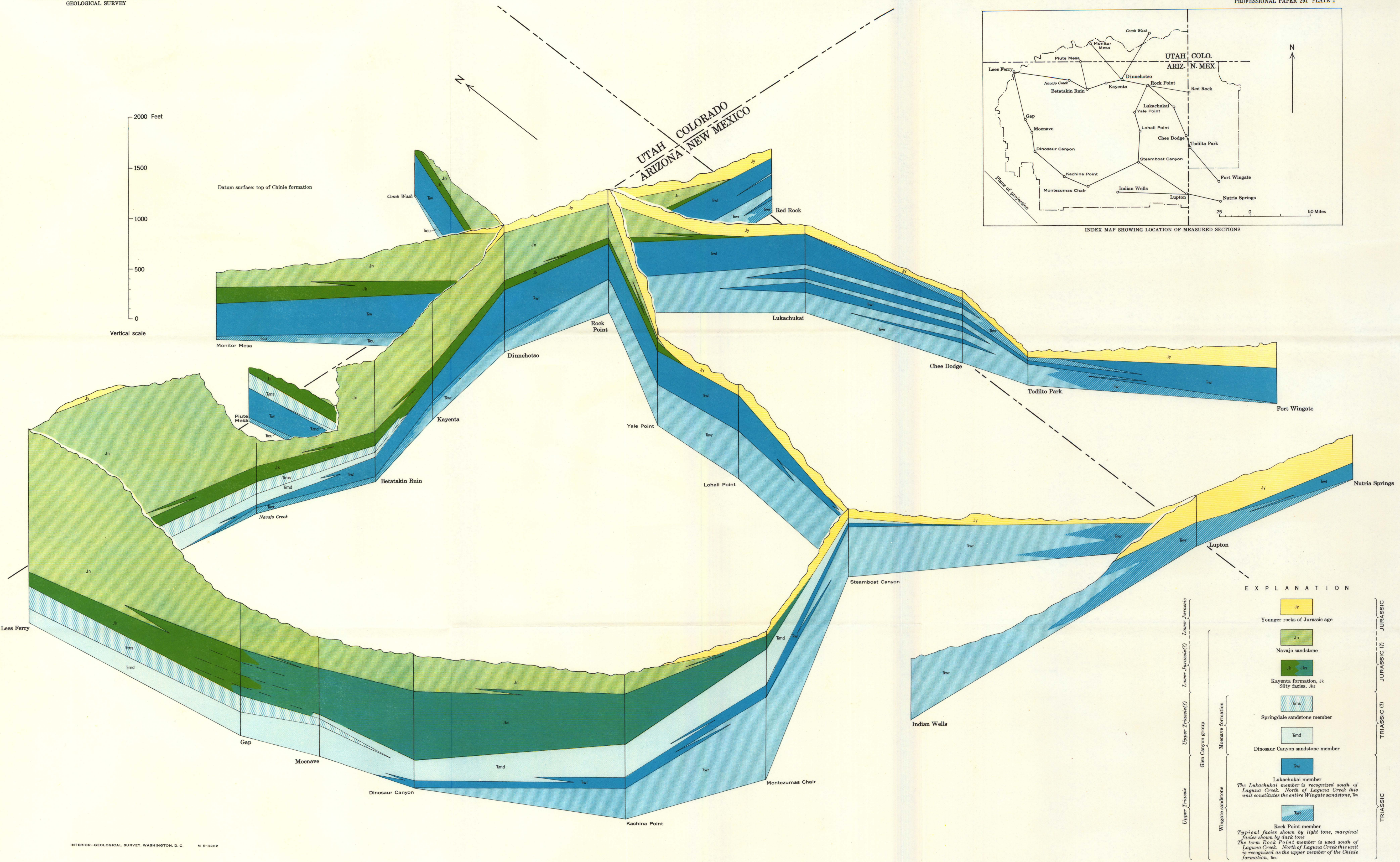
FENCE DIAGRAM OF THE GLEN CANYON GROUP IN THE NAVAJO COUNTRY, ARIZONA, NEW MEXICO, AND UTAH
