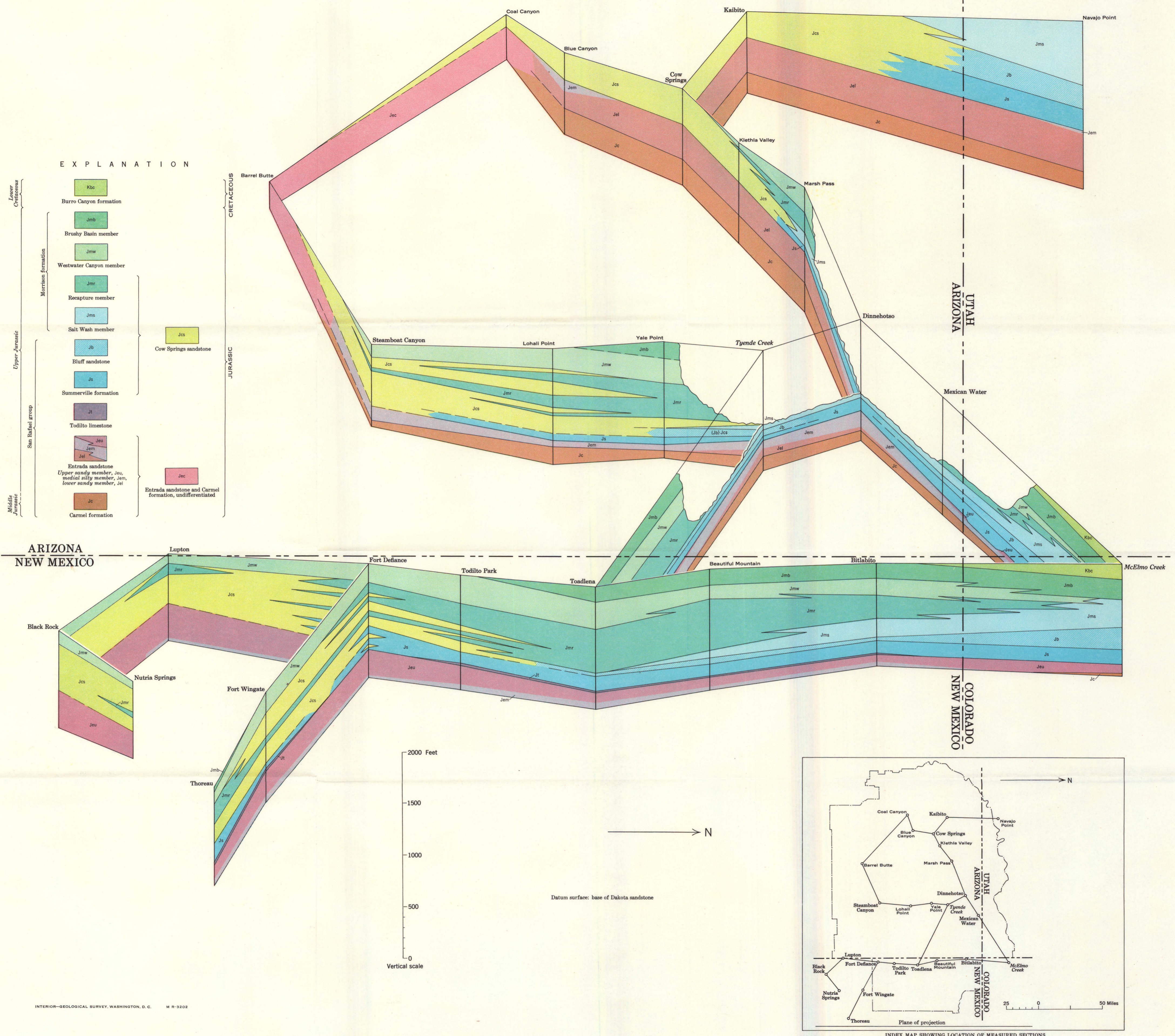
FENCE DIAGRAM OF THE MIDDLE AND UPPER JURASSIC AND LOWER CRETACEOUS ROCKS IN THE NAVAJO COUNTRY, ARIZONA, COLORADO, NEW MEXICO, AND UTAH
