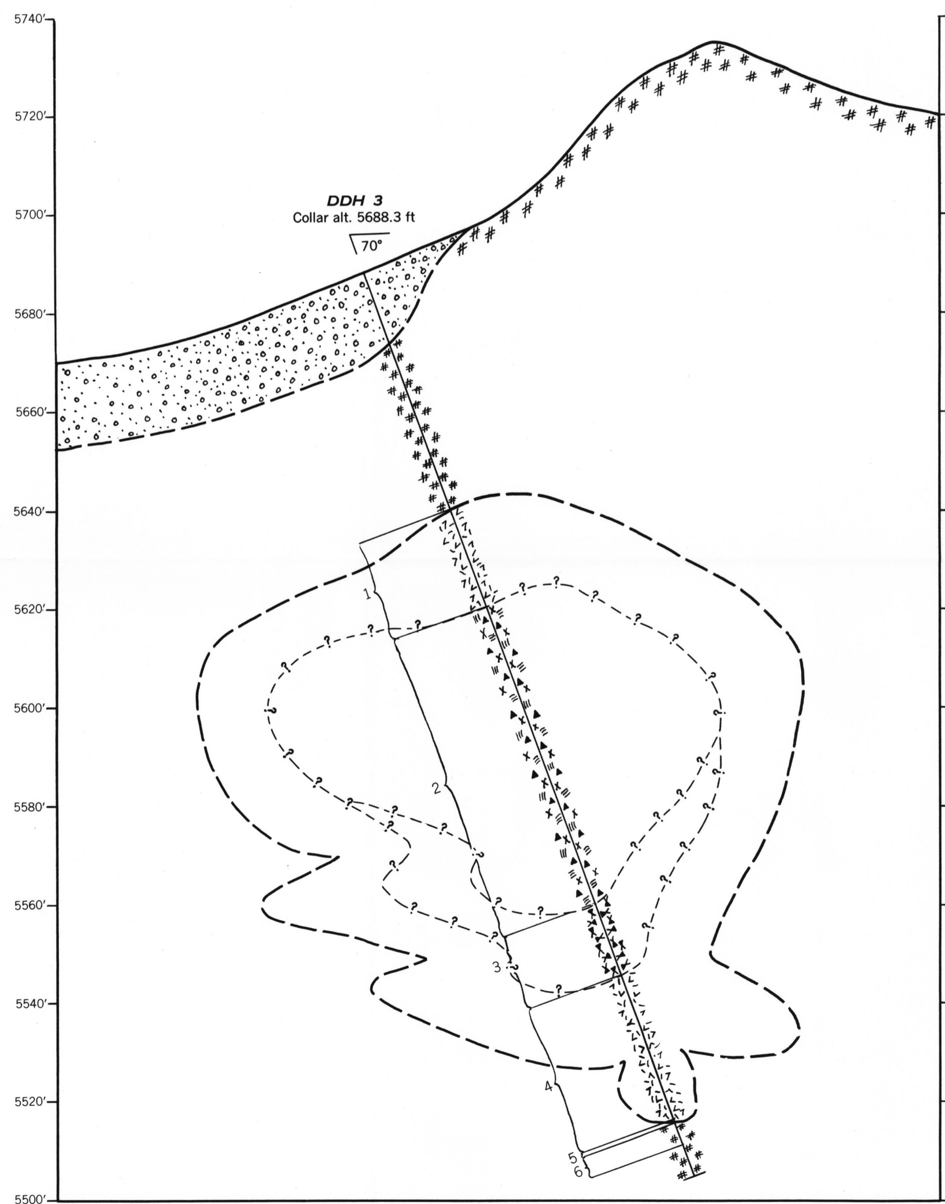
GEOLOGIC SECTIONS THROUGH DIAMOND-DRILL HOLES 1, 2, 3, AND SECTION E-E', TIN MOUNTAIN PEGMATITE, CUSTER COUNTY, SOUTH DAKOTA
