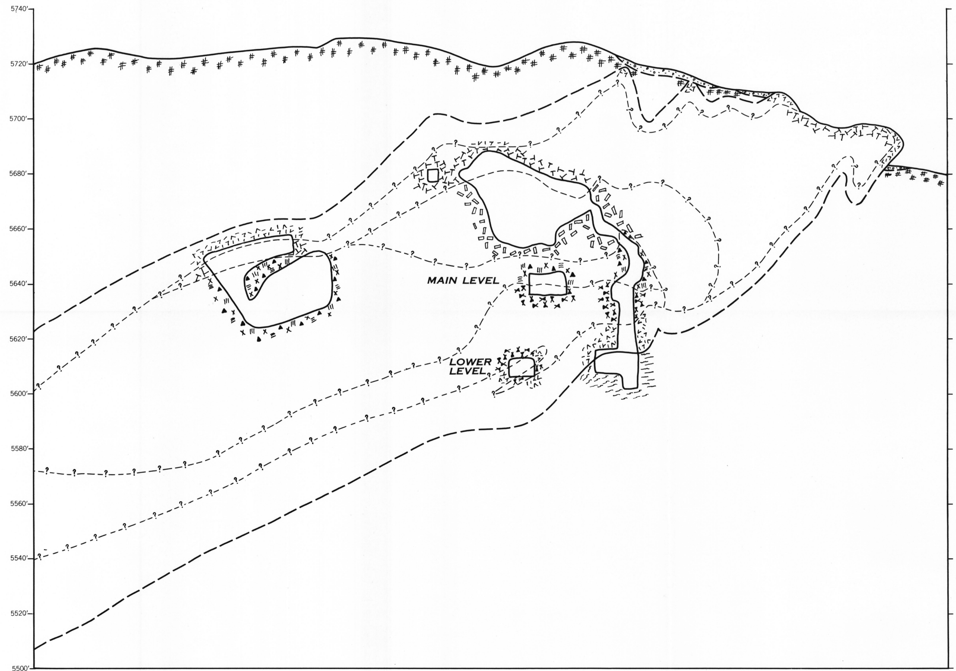
GEOLOGIC SECTIONS THROUGH DIAMOND-DRILL HOLES 1, 2, 3, AND SECTION E-E', TIN MOUNTAIN PEGMATITE, CUSTER COUNTY, SOUTH DAKOTA
