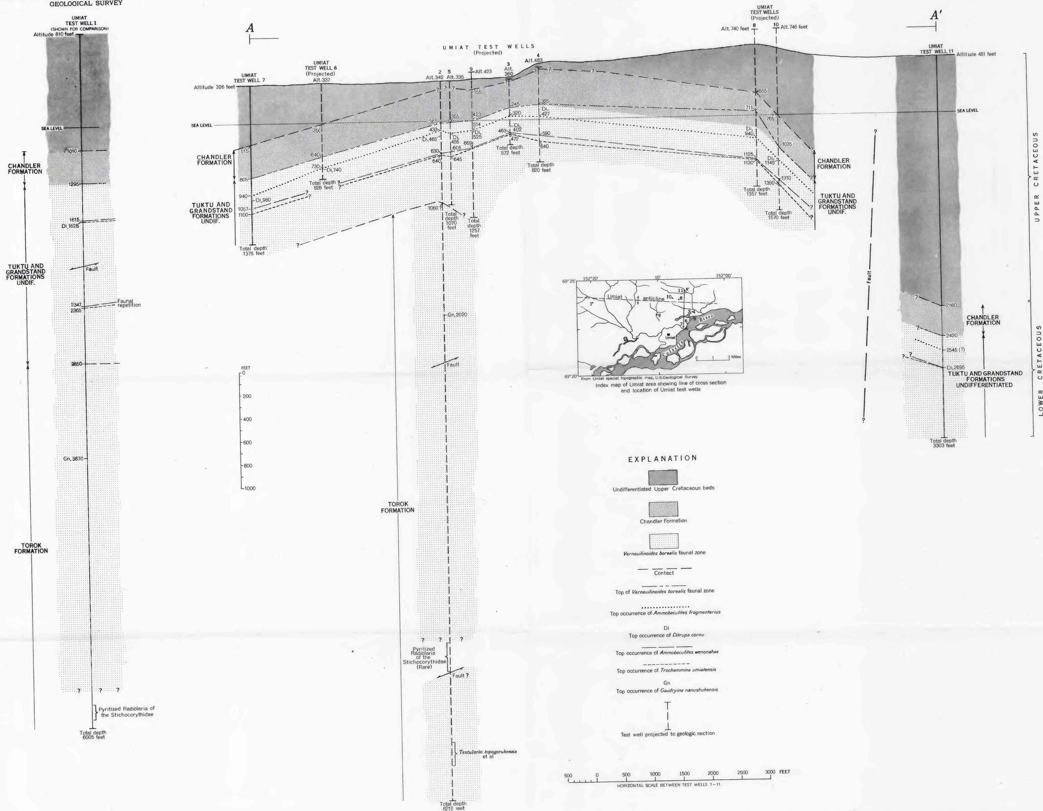
MICROFOSSIL HORIZONS WITHIN VERNEUILINOIDES BOREALIS FAUNAL ZONE IN TEST WELLS 1-11, UMIAT FIELD, NORTHERN ALASKA
