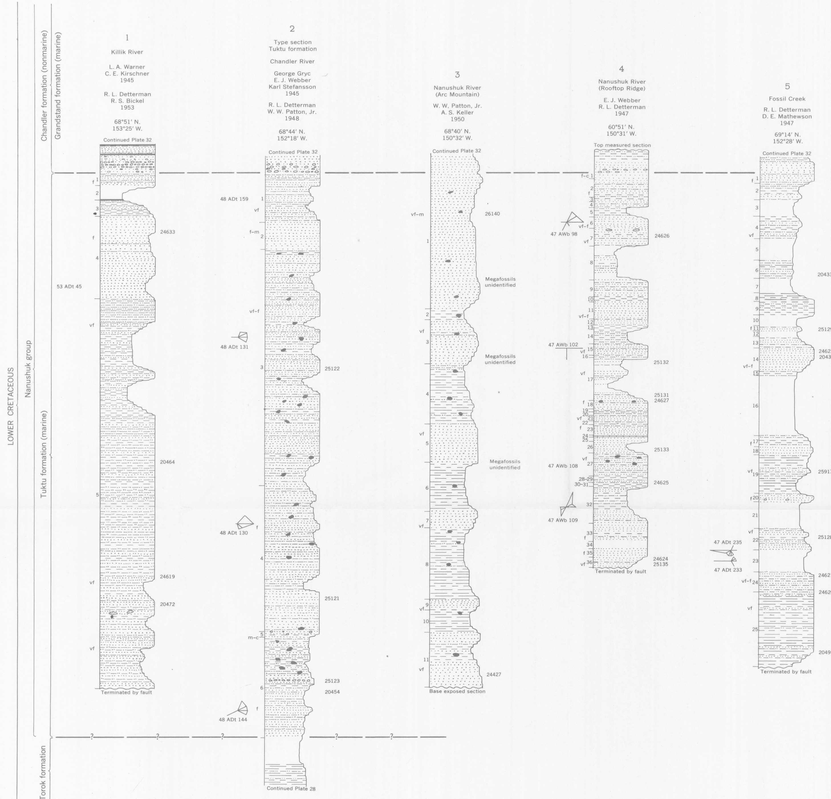
CORRELATED COLUMNAR SECTIONS OF THE TUKTU FORMATION
