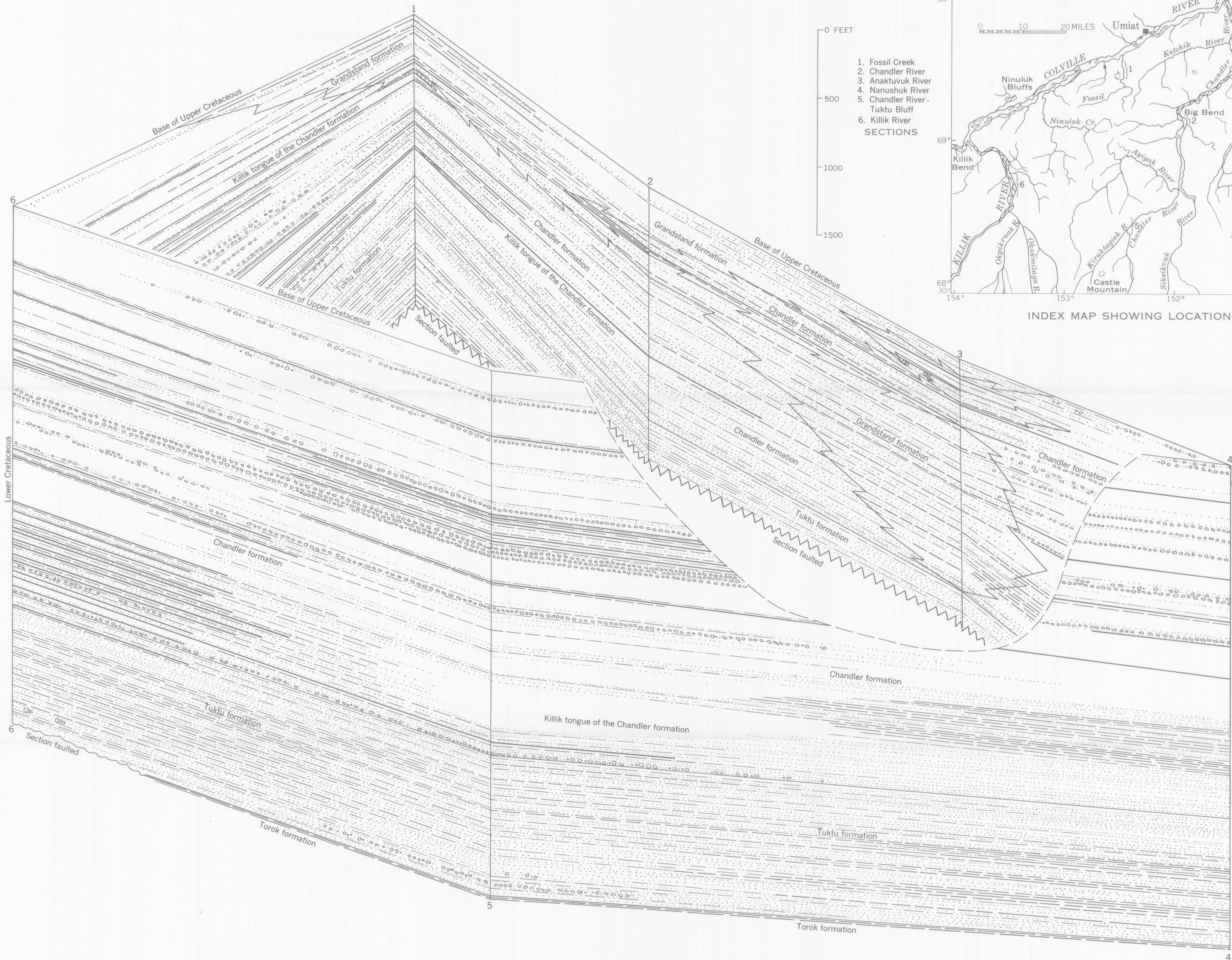
FENCE DIAGRAM OF THE TUKTU, CHANDLER, AND GRANDSTAND FORMATIONS
