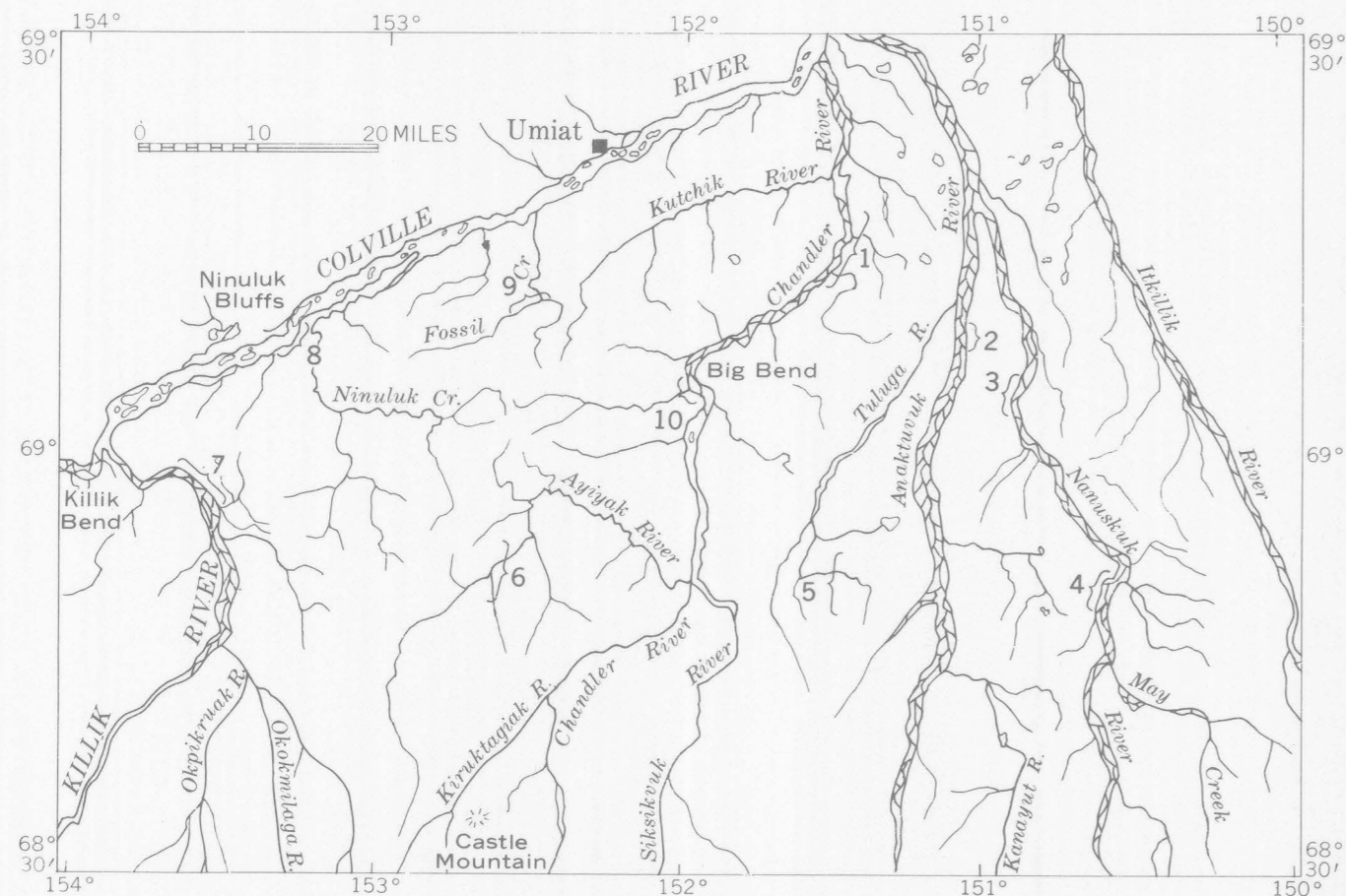
INDEX MAP SHOWING LOCATION OF SECTIONS
