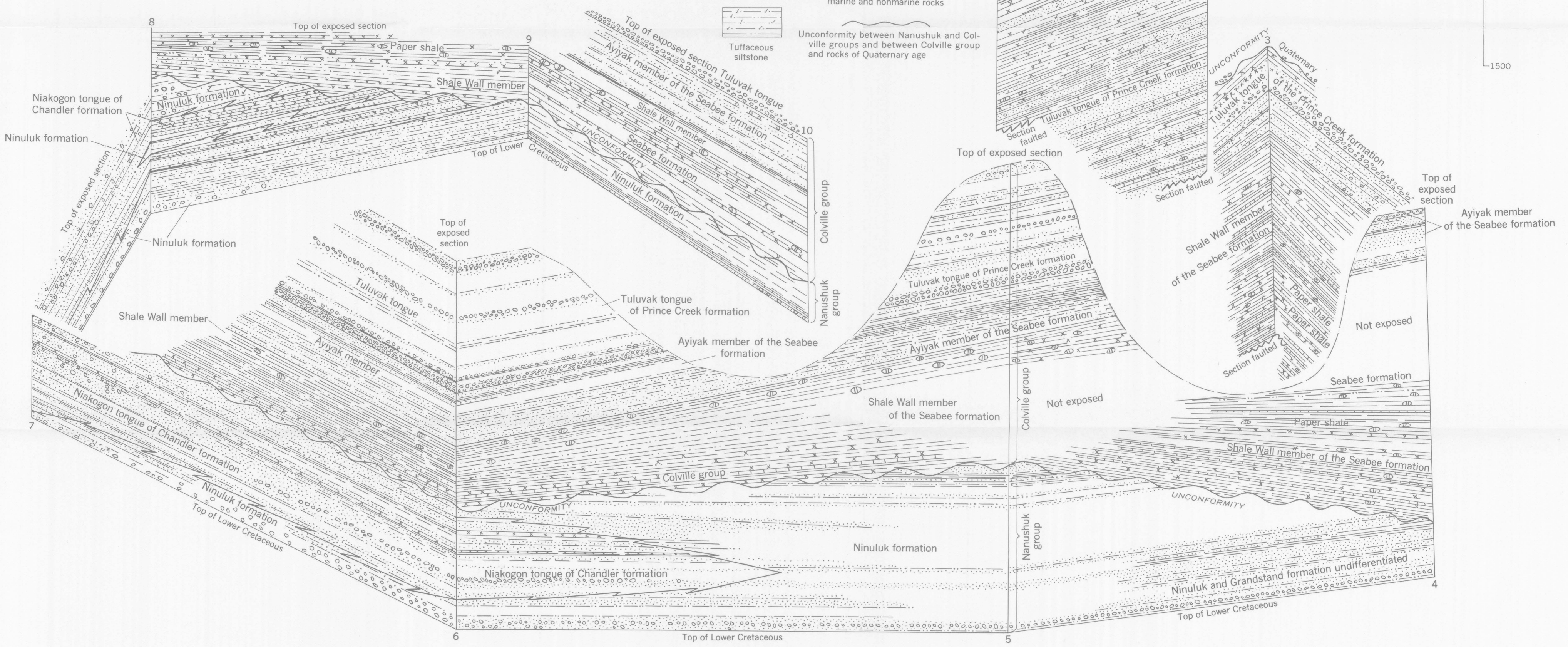
FENCE DIAGRAM OF THE UPPER CRETACEOUS FORMATIONS
