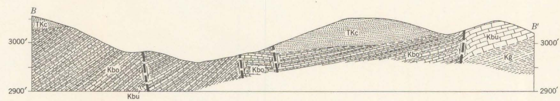
GEOLOGIC MAP AND SECTIONS, FRESNO MINE AREA, TERLINGUA QUICKSILVER DISTRICT, BREWSTER COUNTY, TEXAS
