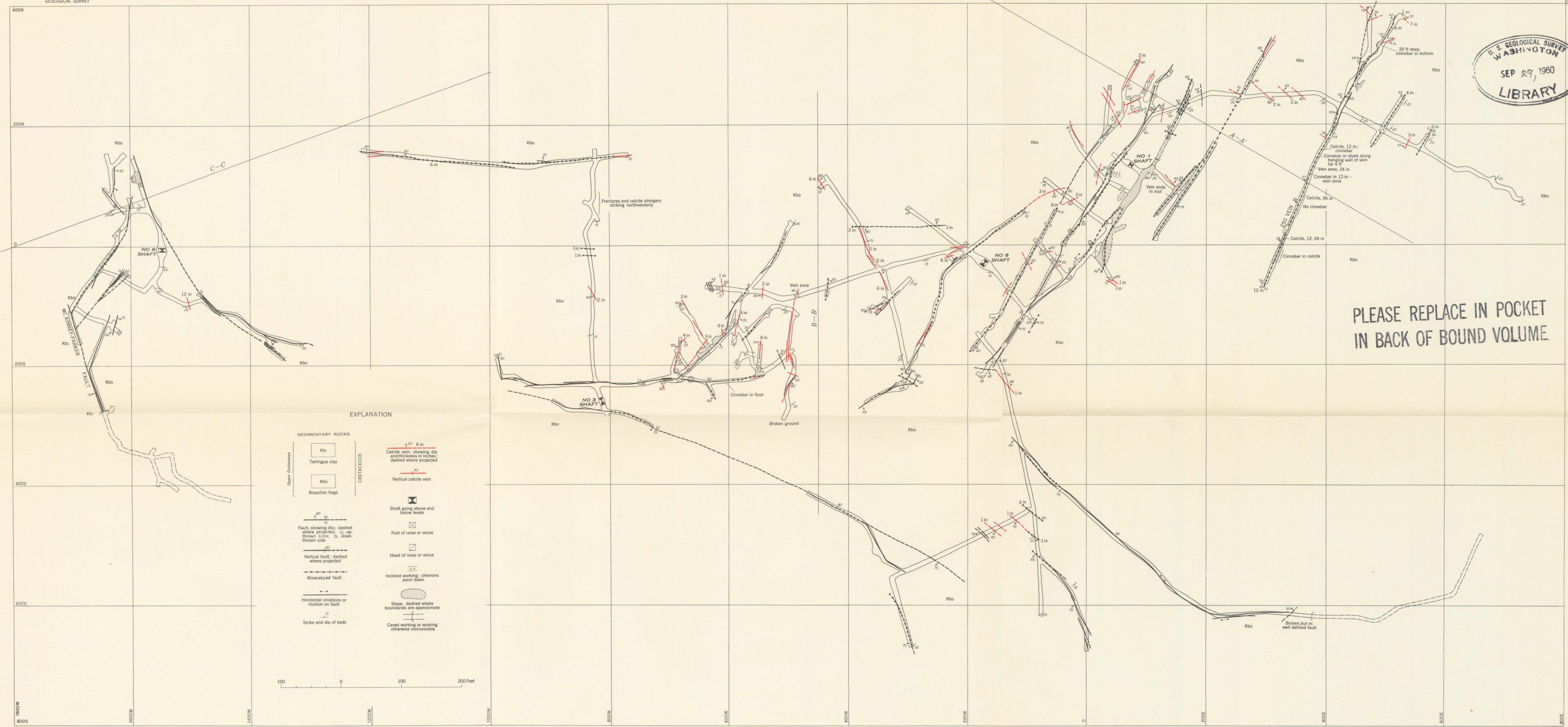
GEOLOGIC MAP OF 250 LEVEL, CHISOS MINE, TERLINGUA QUICKSILVER DISTRICT, BREWSTER COUNTY, TEXAS
