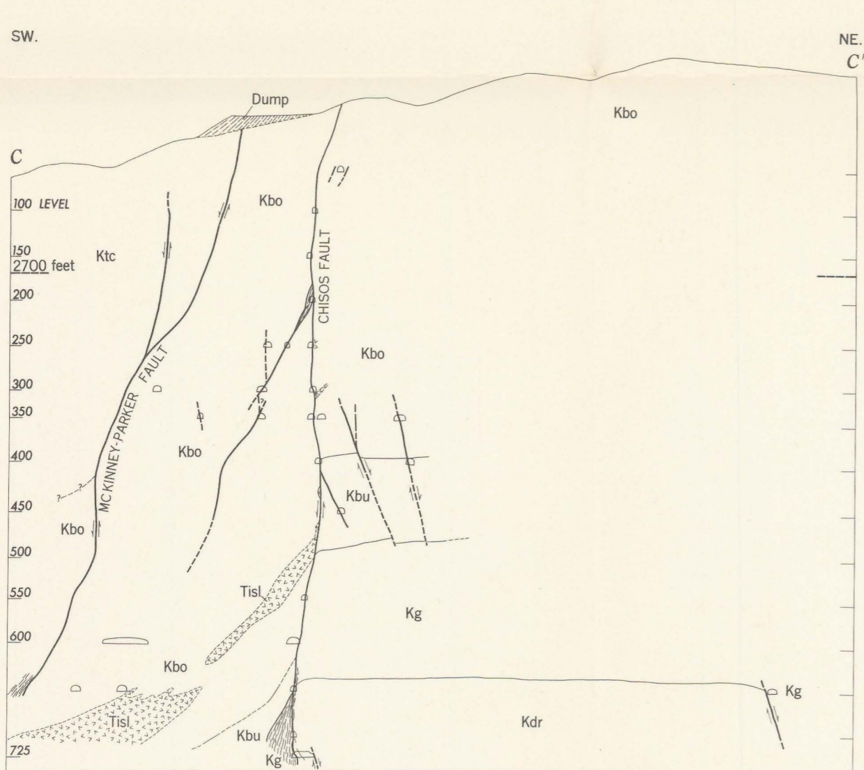
GEOLOGIC SECTIONS OF THE CHISOS MINE, TERLINGUA QUICKSILVER DISTRICT, BREWSTER COUNTY, TEXAS
