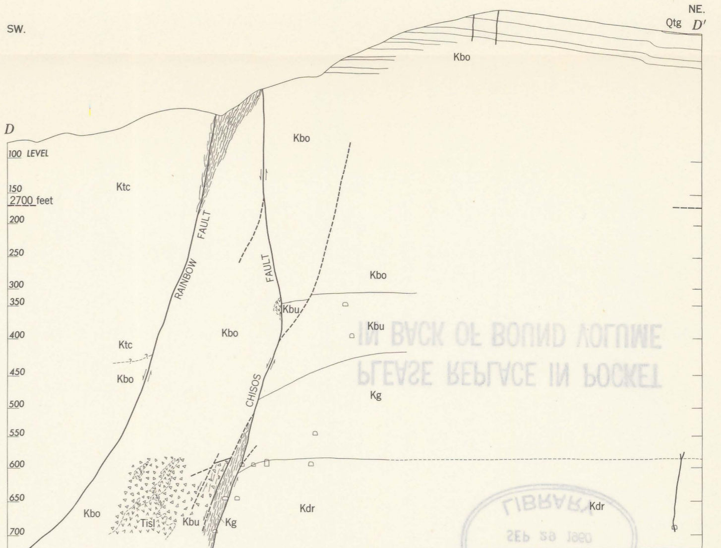
GEOLOGIC SECTIONS OF THE CHISOS MINE, TERLINGUA QUICKSILVER DISTRICT, BREWSTER COUNTY, TEXAS
