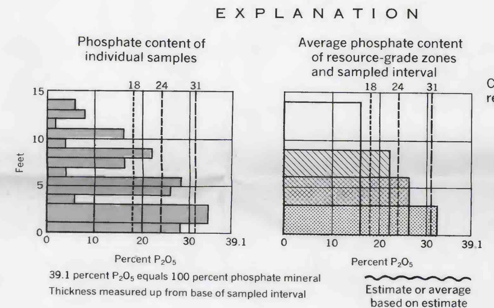
GRAPHS SHOWING STRATIGRAPHIC DISTRIBUTION OF PHOSPHATE WITHIN THE RETORT PHOSPHATIC SHALE MEMBER OF BIOSPIRIFERA FORMATION IN CENTRAL AND WESTERN MONTANA
