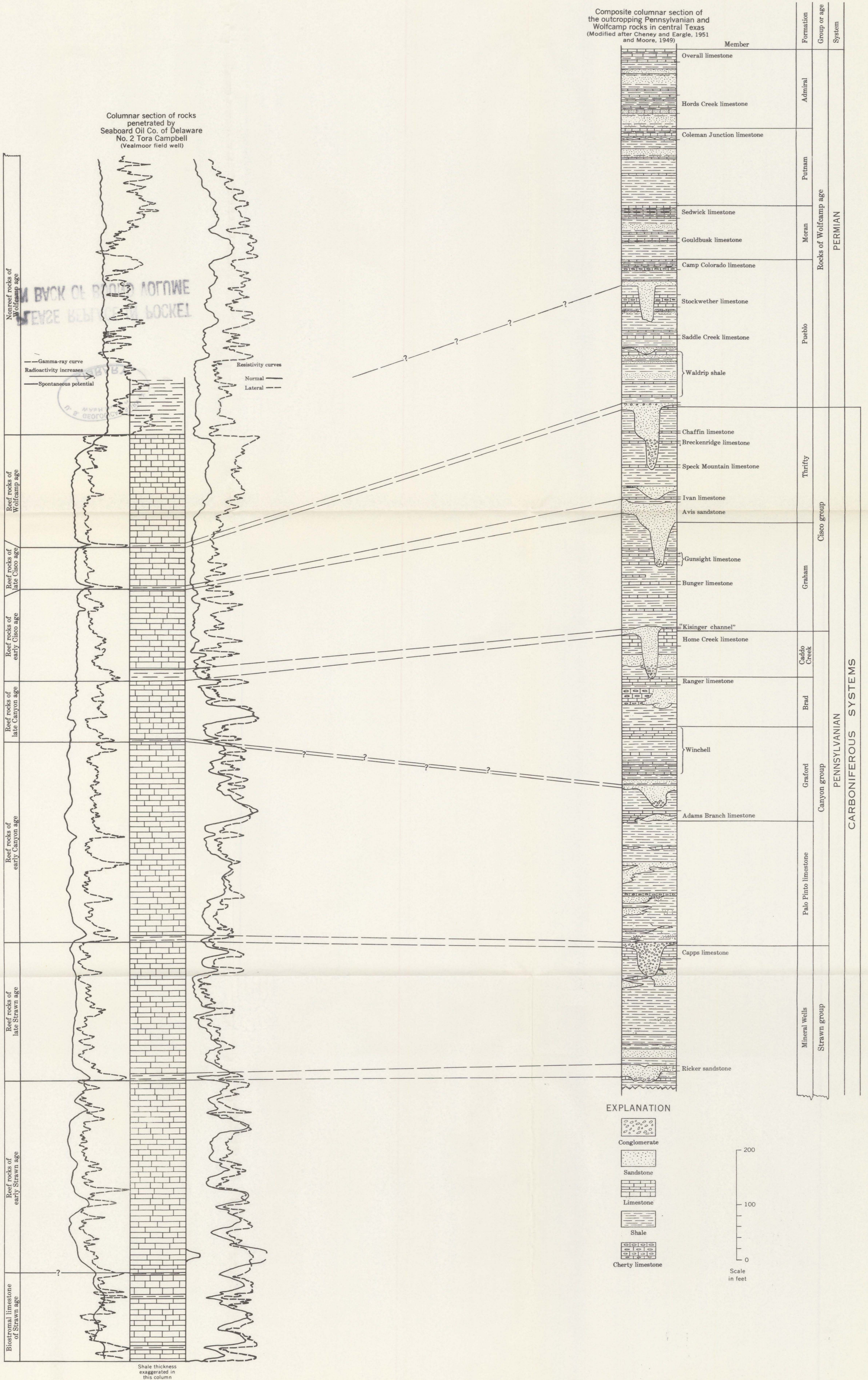
POSSIBLE CORRELATION BETWEEN UNCONFORMITIES IN THE HORSESHOE ATOLL AND OUTCROPPING ROCKS IN CENTRAL TEXAS
