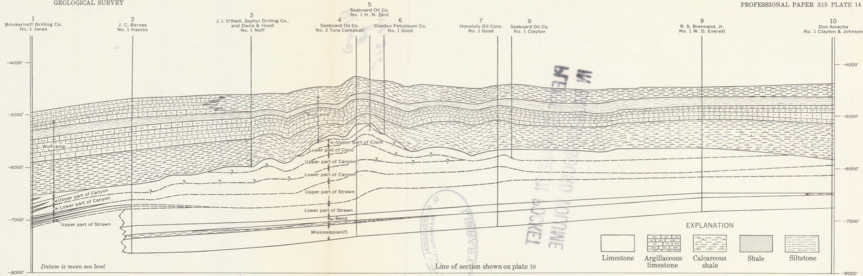
SECTION SHOWING STRATIGRAPHIC RELATIONSHIPS OF THE ROCKS OF PRE-LEONARD AND POST-DEVONIAN AGE PENETRATED BY WELLS IN BORDEN AND HOWARD COUNTIES, TEXAS
