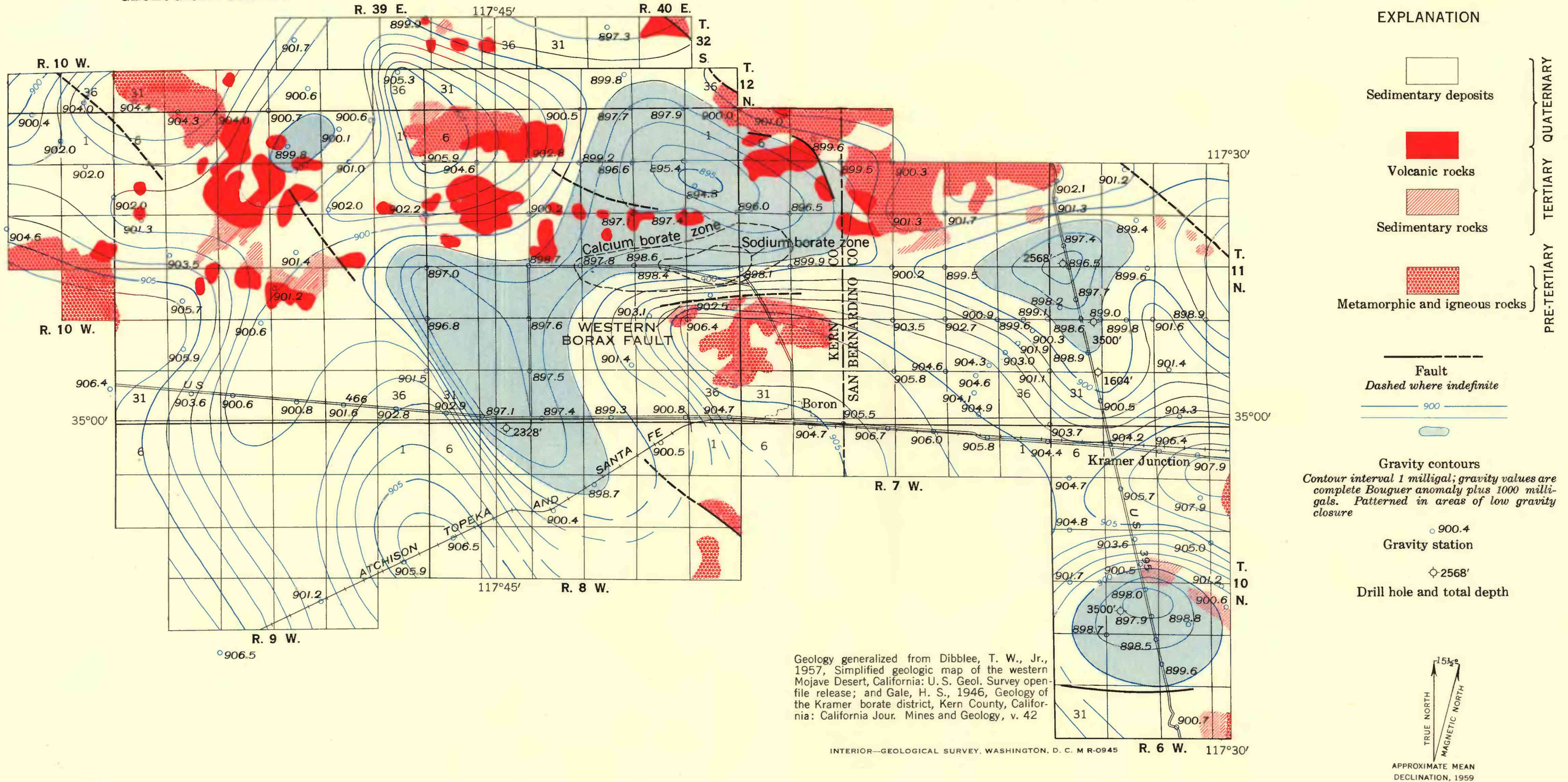
BOUGUER ANOMALY AND GENERALIZED GEOLOGIC MAP OF THE AREA IN THE VICINITY OF THE KRAMER BORATE DISTRICT, CALIFORNIA
