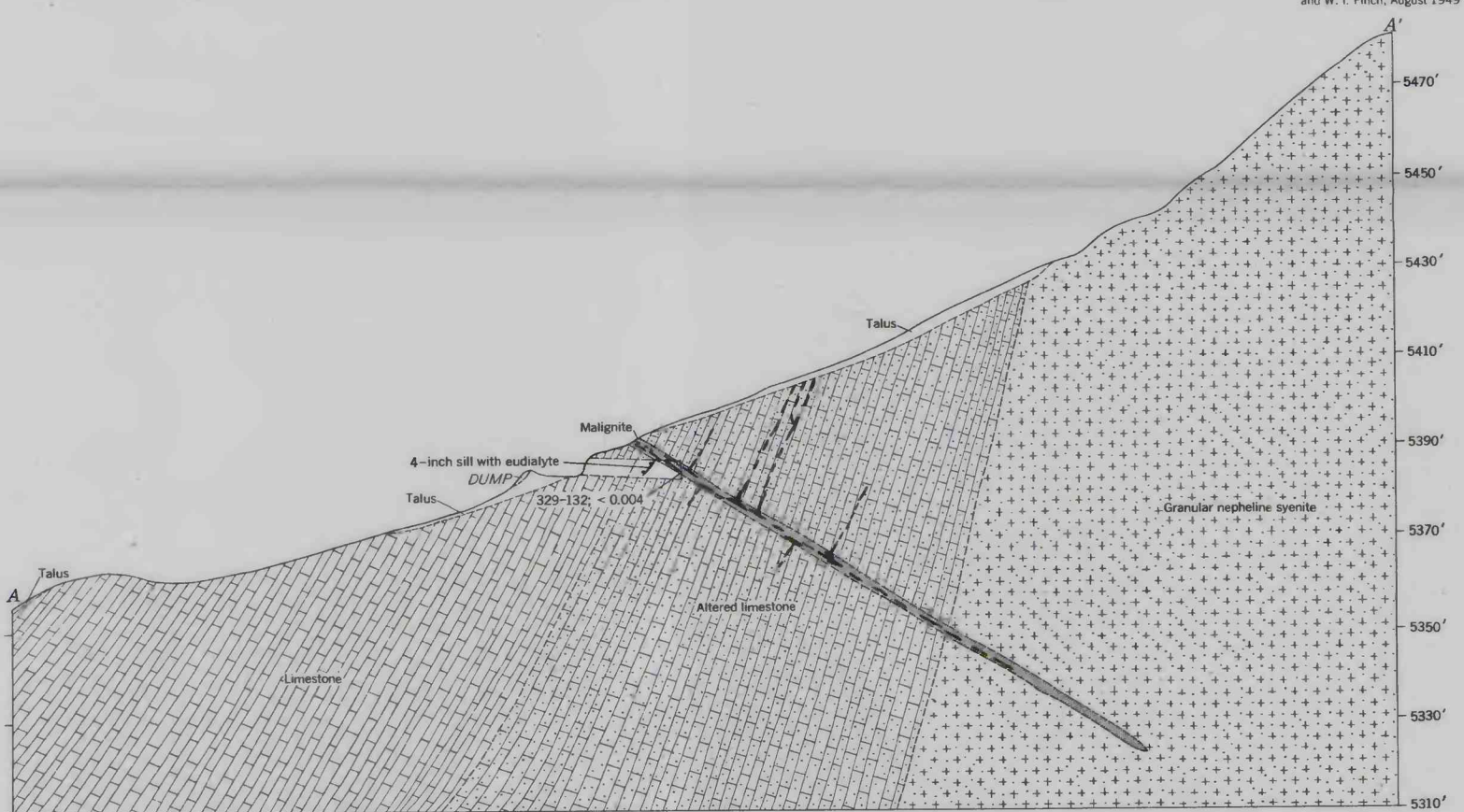
GEOLOGIC MAP AND SECTION OF WESTERN AREA, WIND MOUNTAIN, OTERO COUNTY, NEW MEXICO
