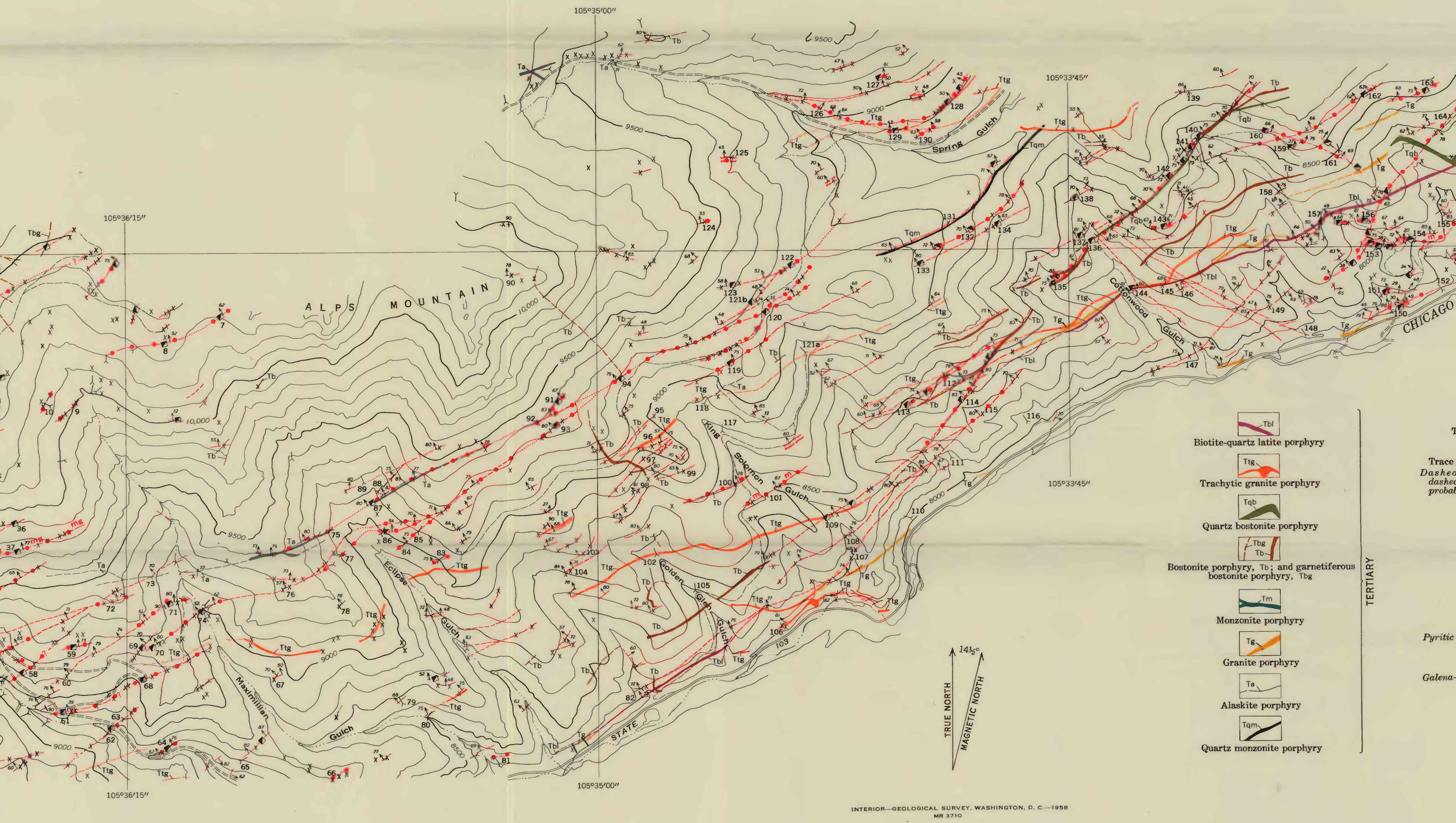
MAP OF THE CHICAGO CREEK AREA SHOWING THE LOCATION OF MINES AND THE DISTRIBUTION OF VEINS AND DIKE ROCKS
