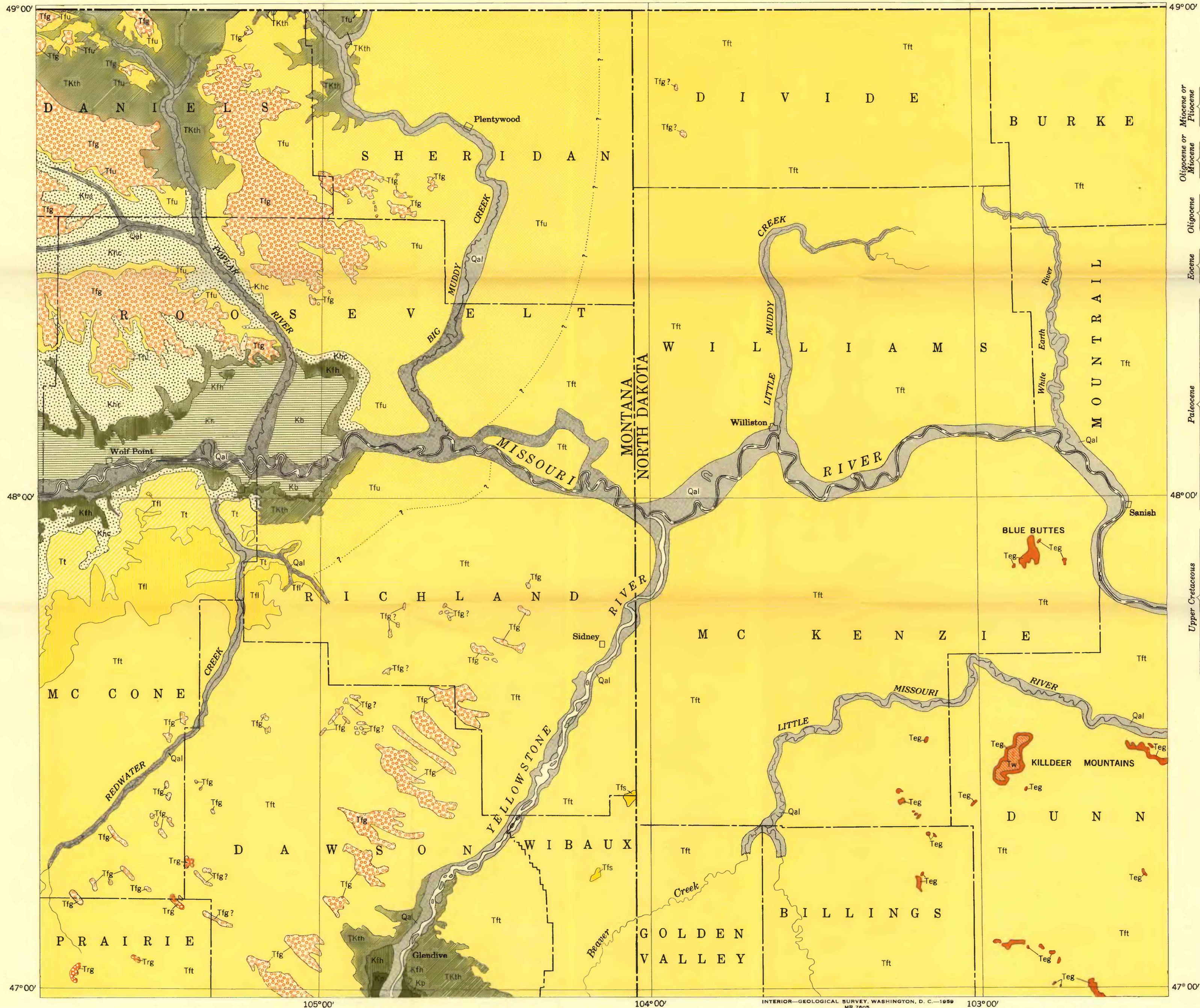
MAP OF PRE-PLEISTOCENE ROCKS OF NORTHEASTERN MONTANA AND NORTHWESTERN NORTH DAKOTA
