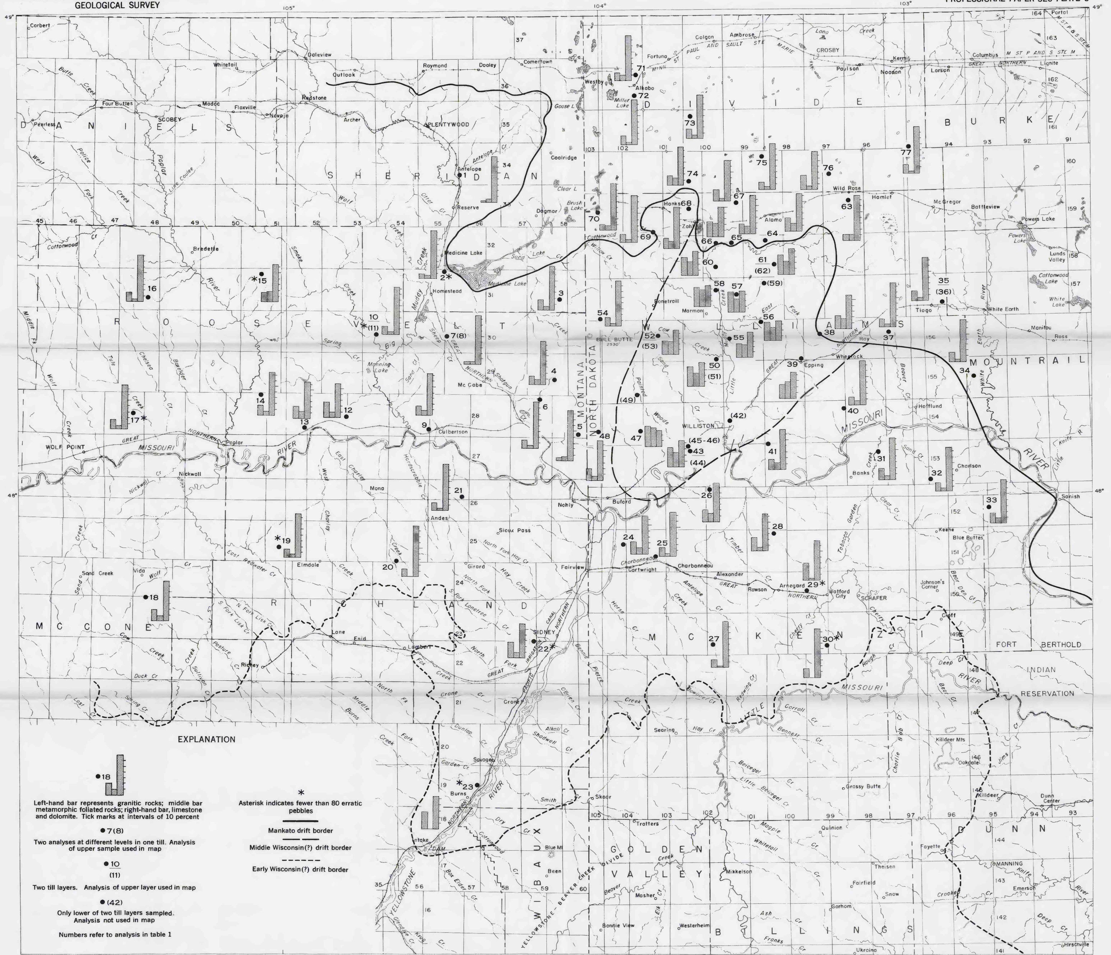
MAP SHOWING HISTOGRAMS OF ERRATIC-PEBBLE CONTENT OF SURFACE TILL, NORTHEASTERN MONTANA AND NORTHWESTERN NORTH DAKOTA
