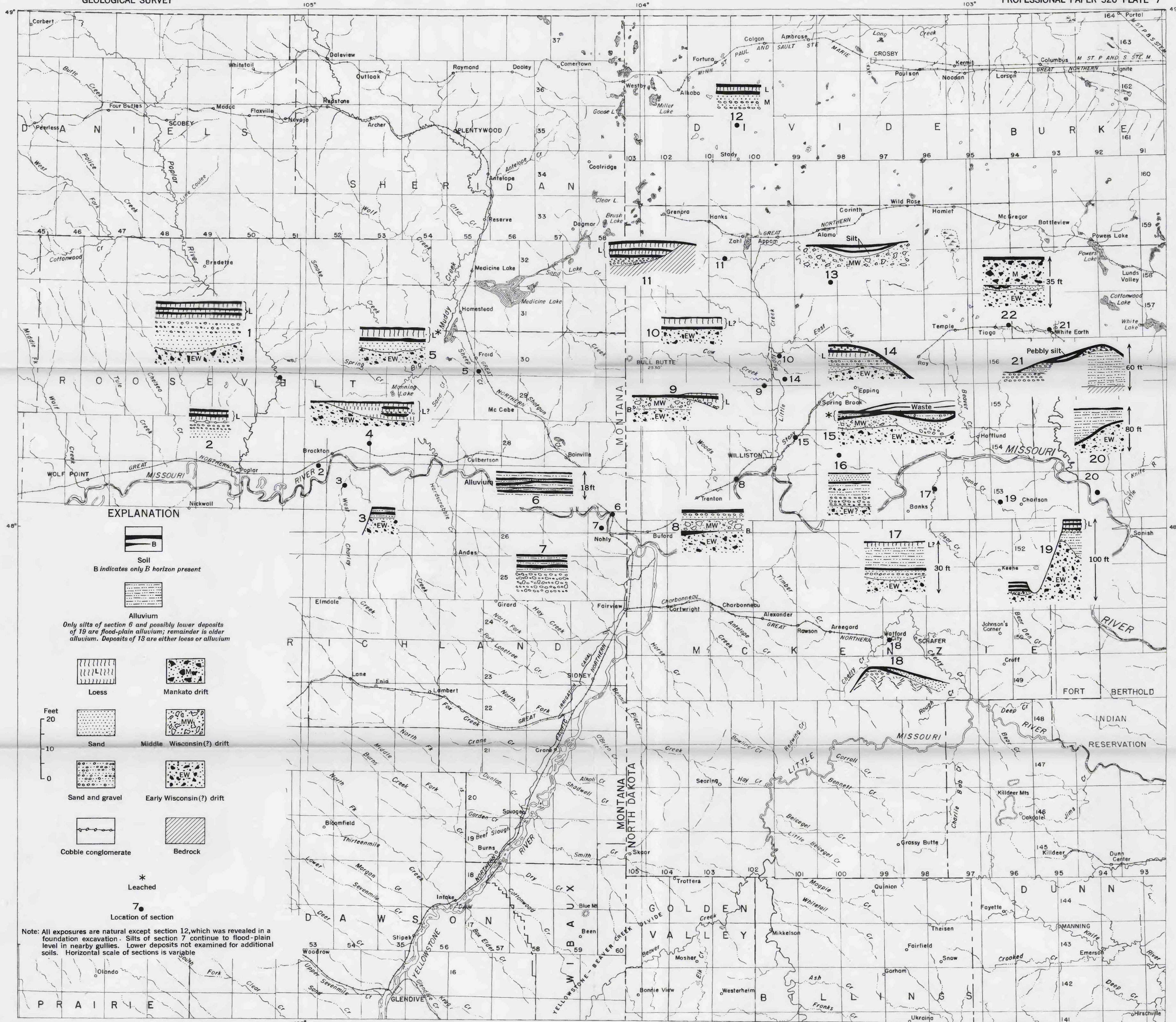
GENERALIZED STRATIGRAPHIC SECTIONS OF MODERN AND FOSSIL SOILS AND LOESS, NORTHEASTERN MONTANA AND NORTHWESTERN NORTH DAKOTA
