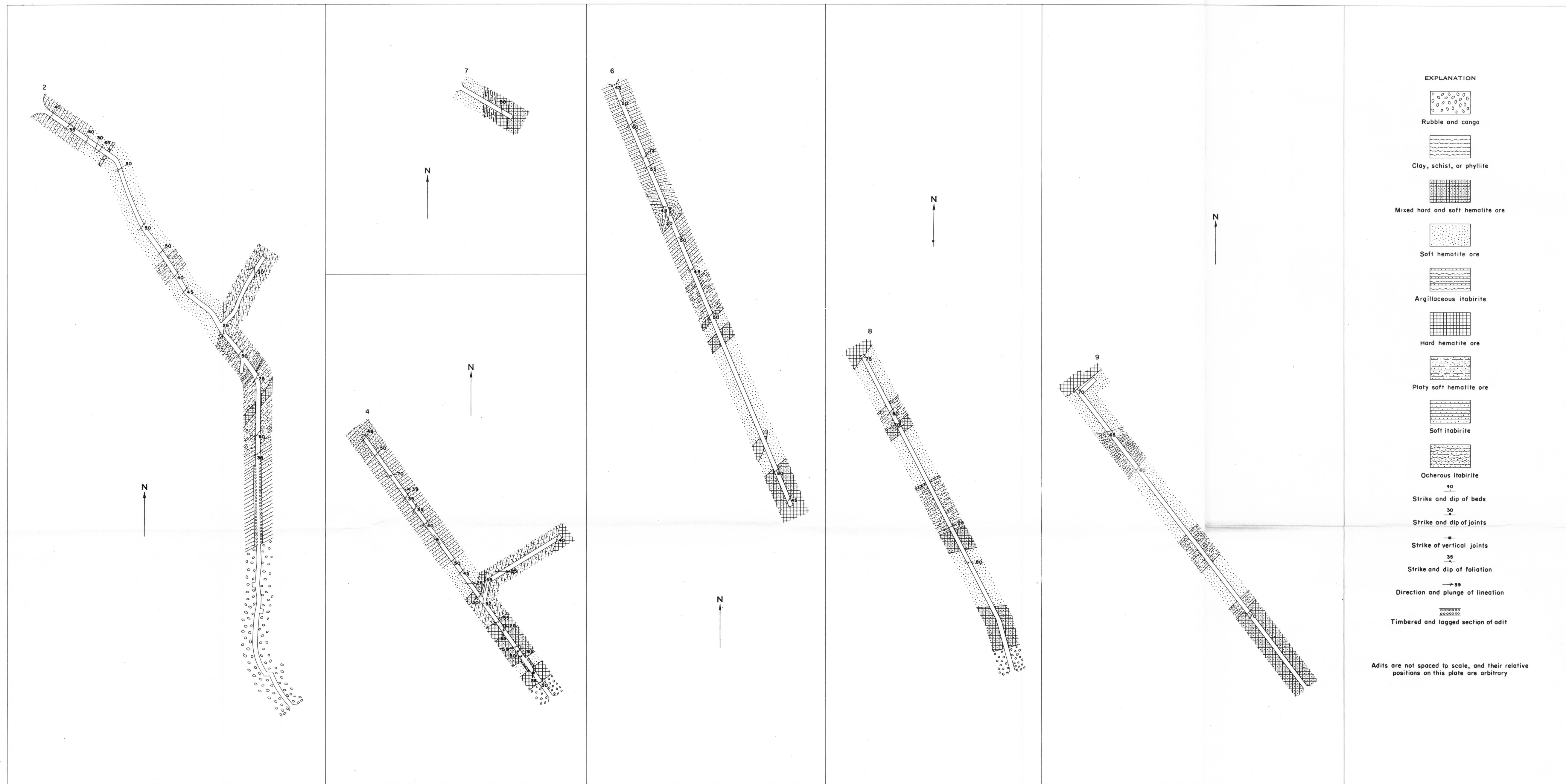
GEOLOGIC MAP OF EXPLORATION ADITS AT ÁGUAS CLARAS, BELO HORIZONTE QUADRANGLE, MINAS GERAIS, BRAZIL
