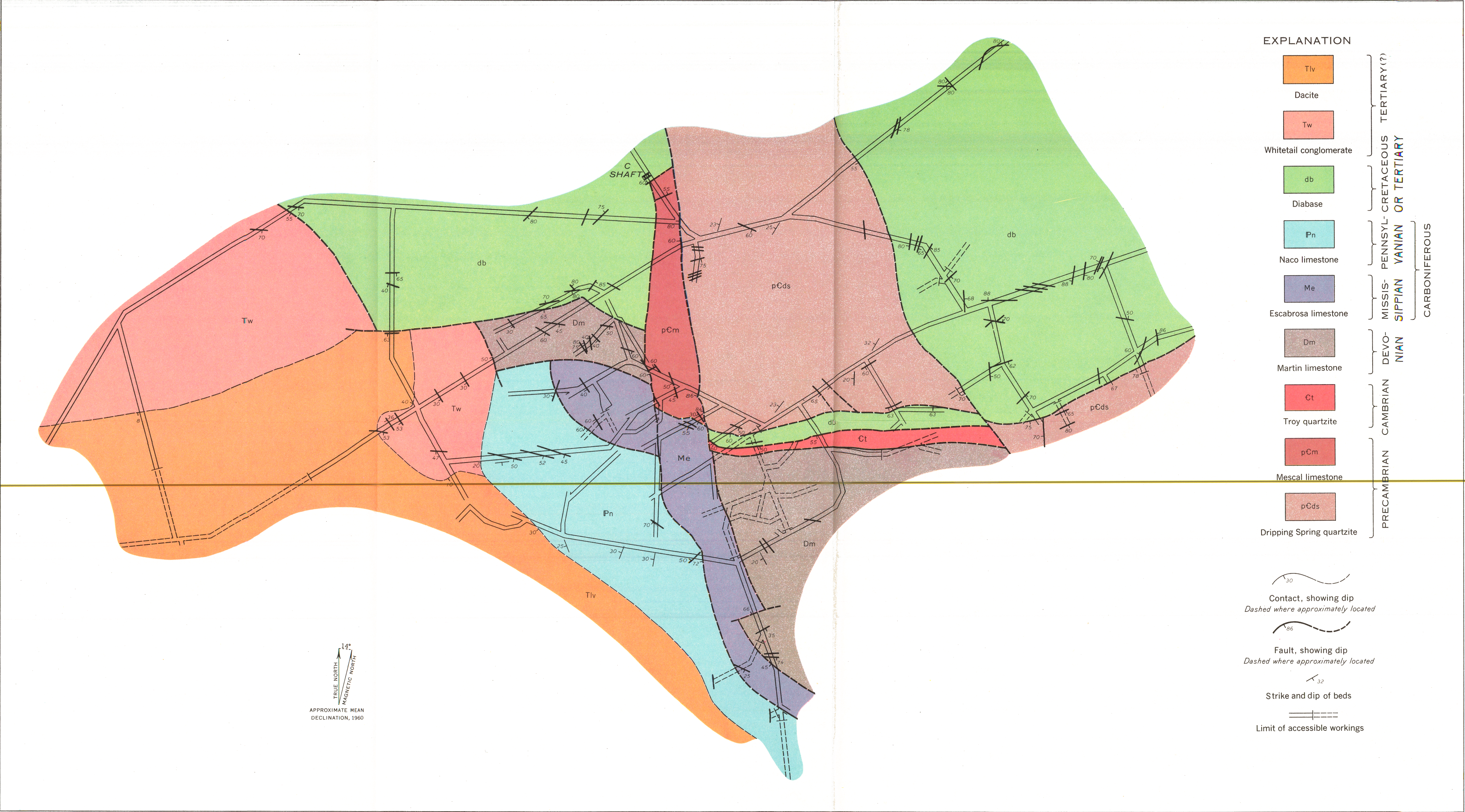
GEOLOGIC MAP OF WEST END OF 12 LEVEL, OLD DOMINION MINE, GLOBE-MIAMI DISTRICT, ARIZONA
