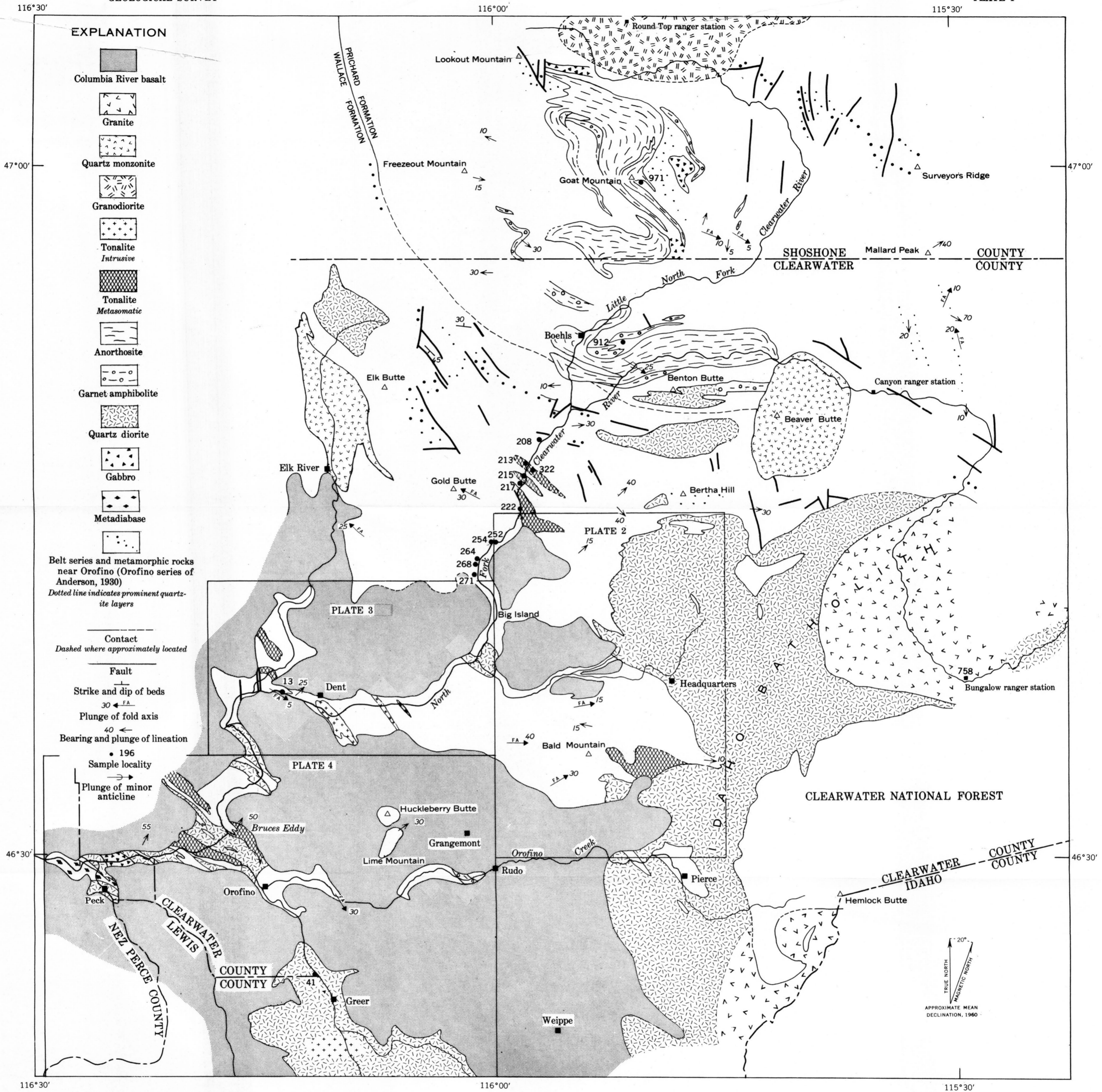
GEOLOGIC SKETCH MAP SHOWING DISTRIBUTION OF INTRUSIVE AND METAMORPHIC ROCKS NORTHWEST OF THE IDAHO BATHOLITH
