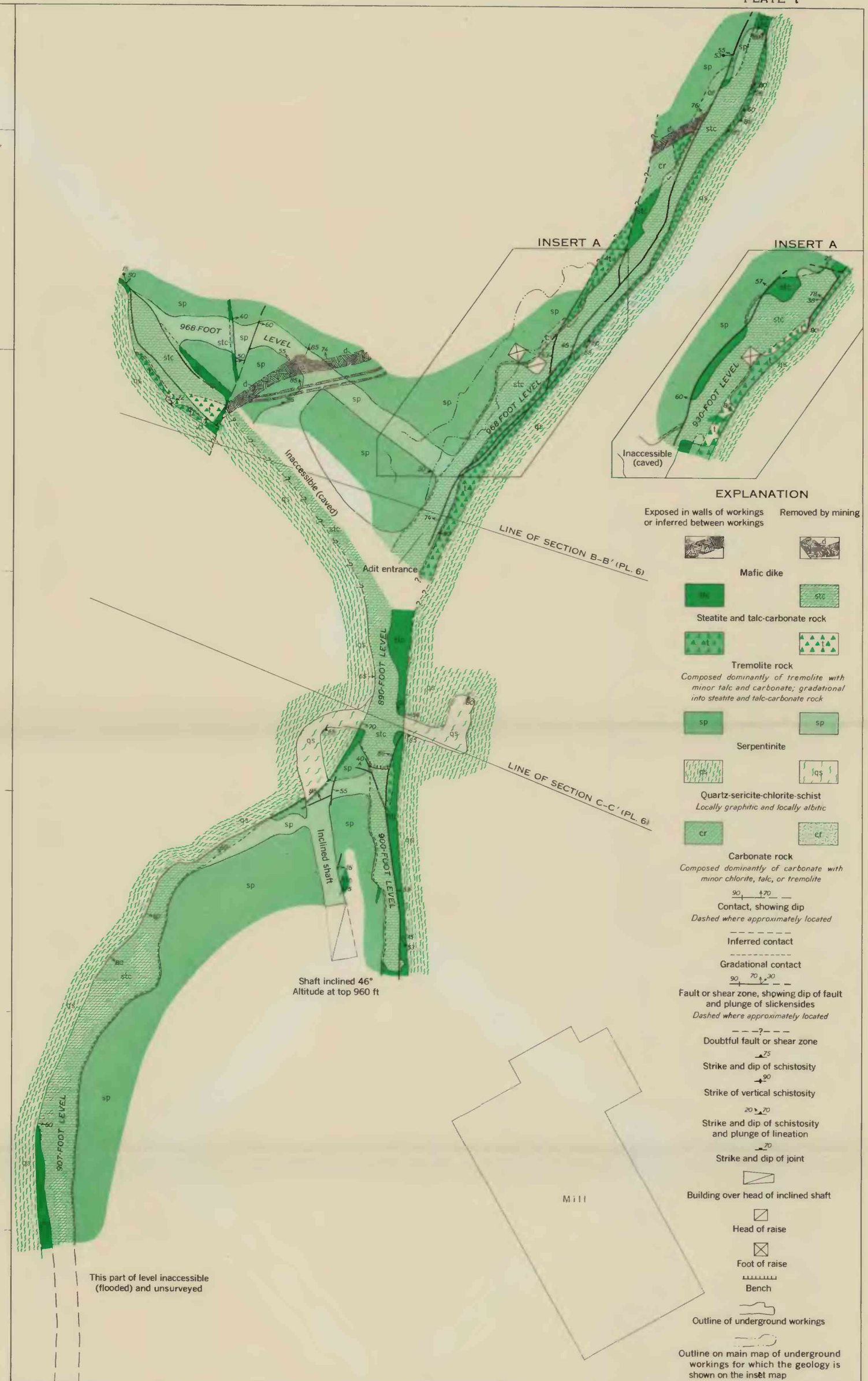
UNDERGROUND GEOLOGIC MAP
