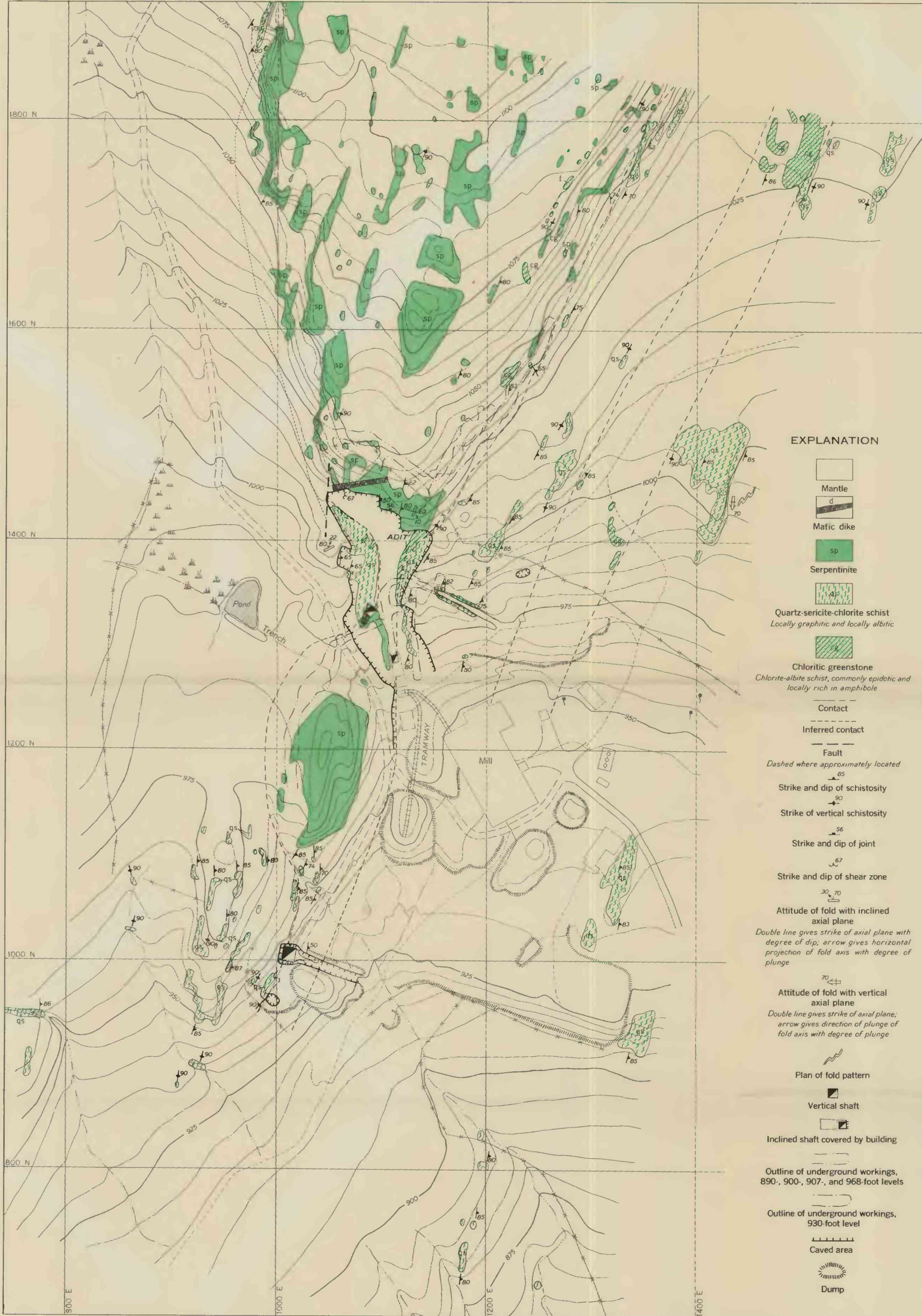
SURFACE GEOLOGIC MAP
