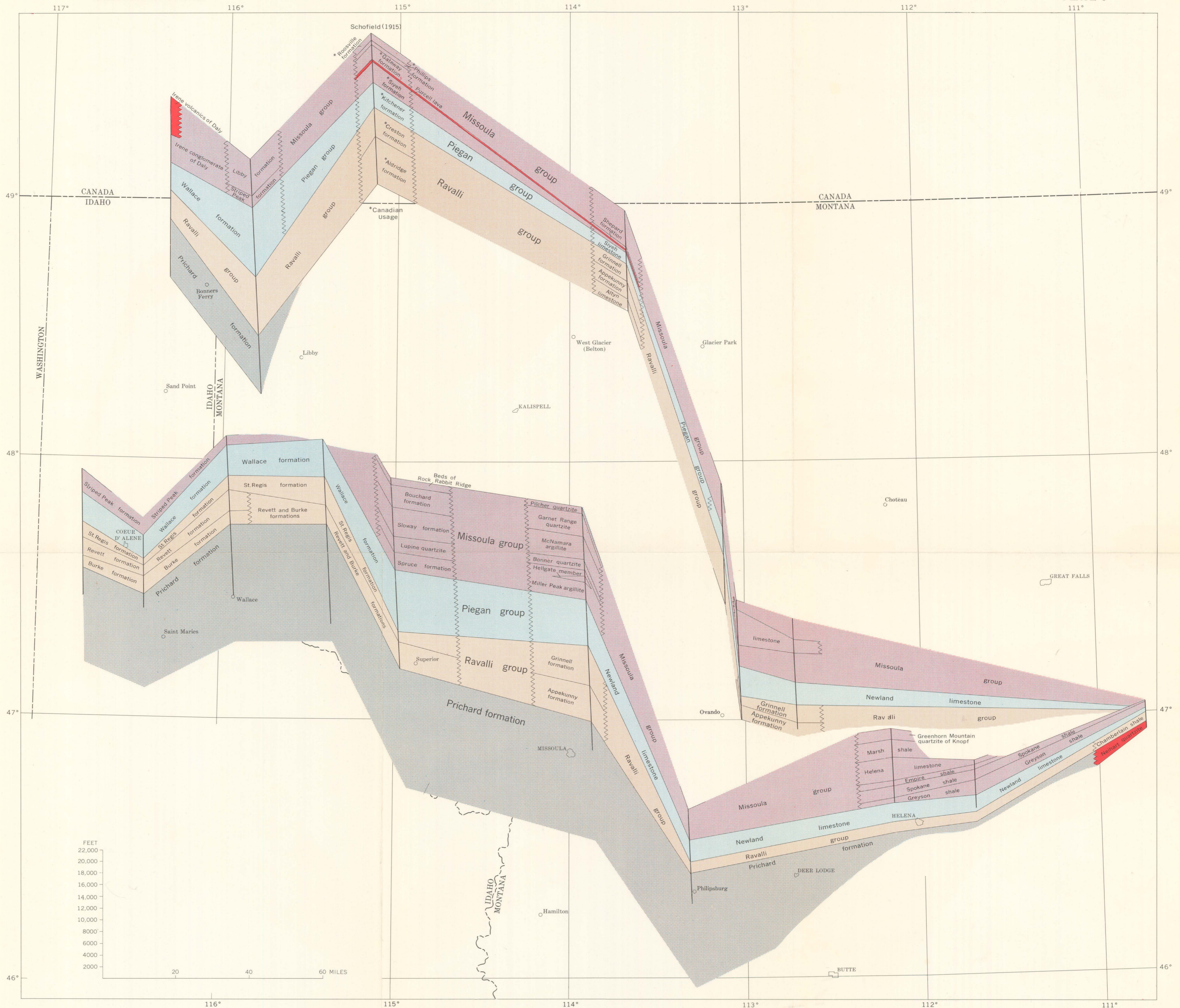
FENCE DIAGRAM SHOWING STRATIGRAPHIC RELATIONS OF THE PRINCIPAL UNITS OF THE BELT SERIES
