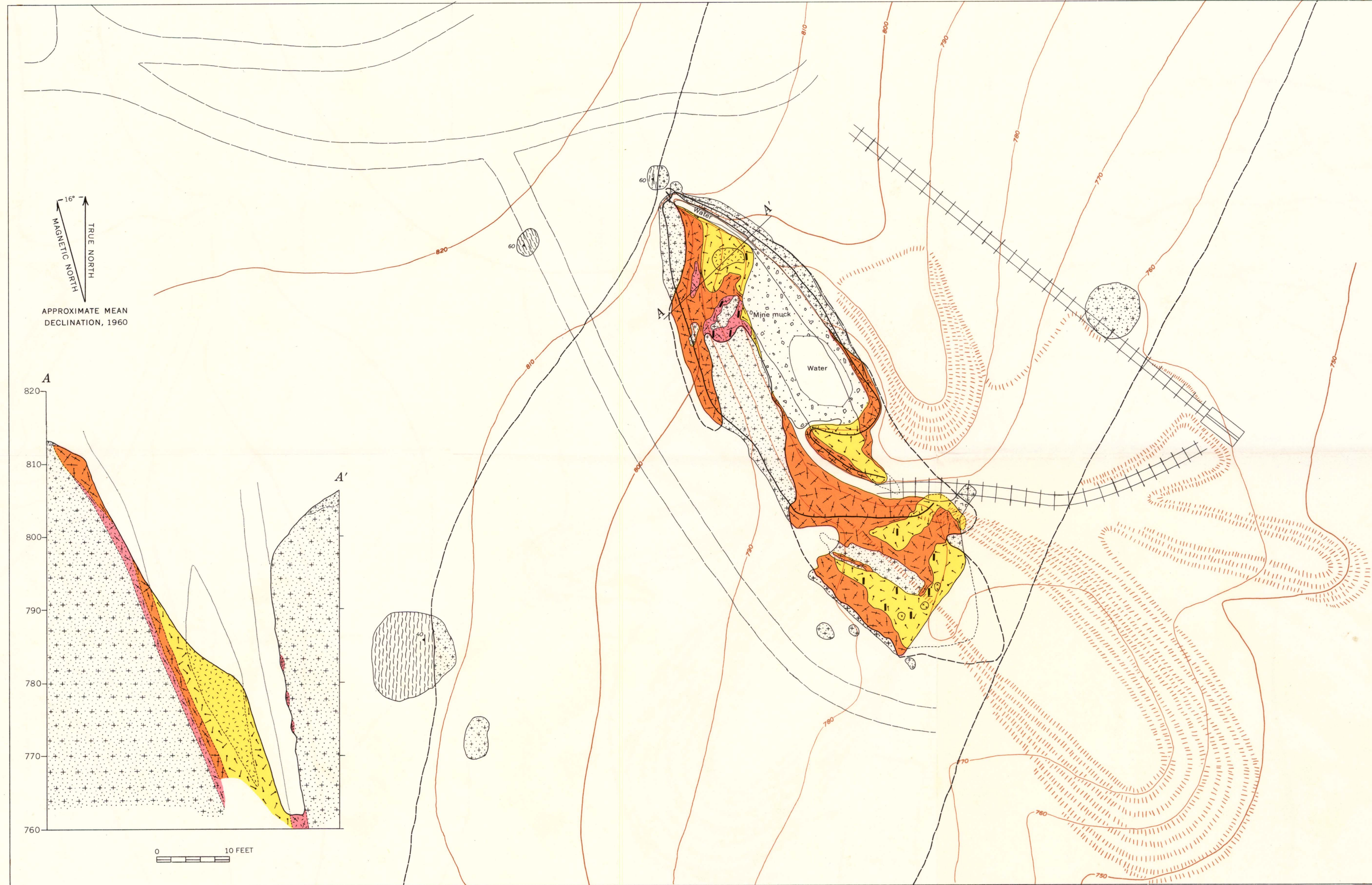
GEOLOGIC MAP AND GENERALIZED SECTION OF THE PARKER MOUNTAIN MINE STRAFFORD, STRAFFORD COUNTY, NEW HAMPSHIRE
