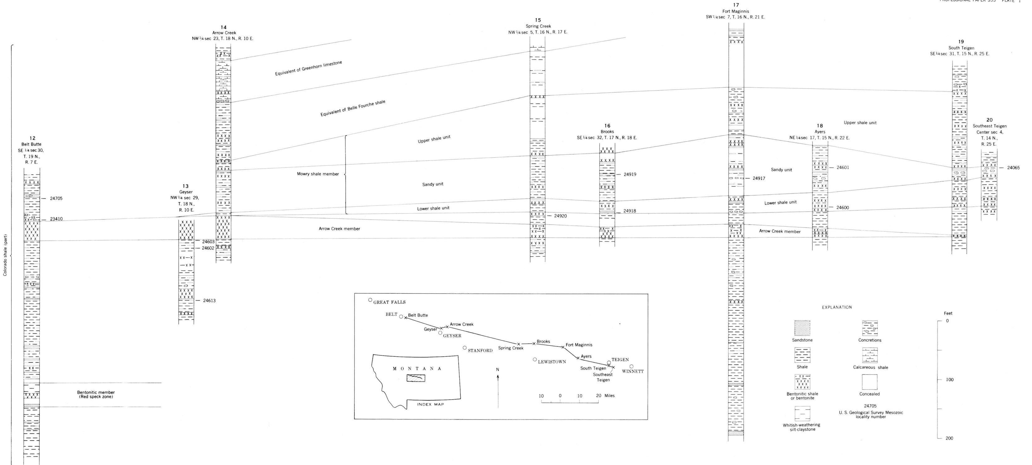
GRAPHIC SECTIONS OF PART OF THE COLORADO SHALE OF NORTH-CENTRAL MONTANA
