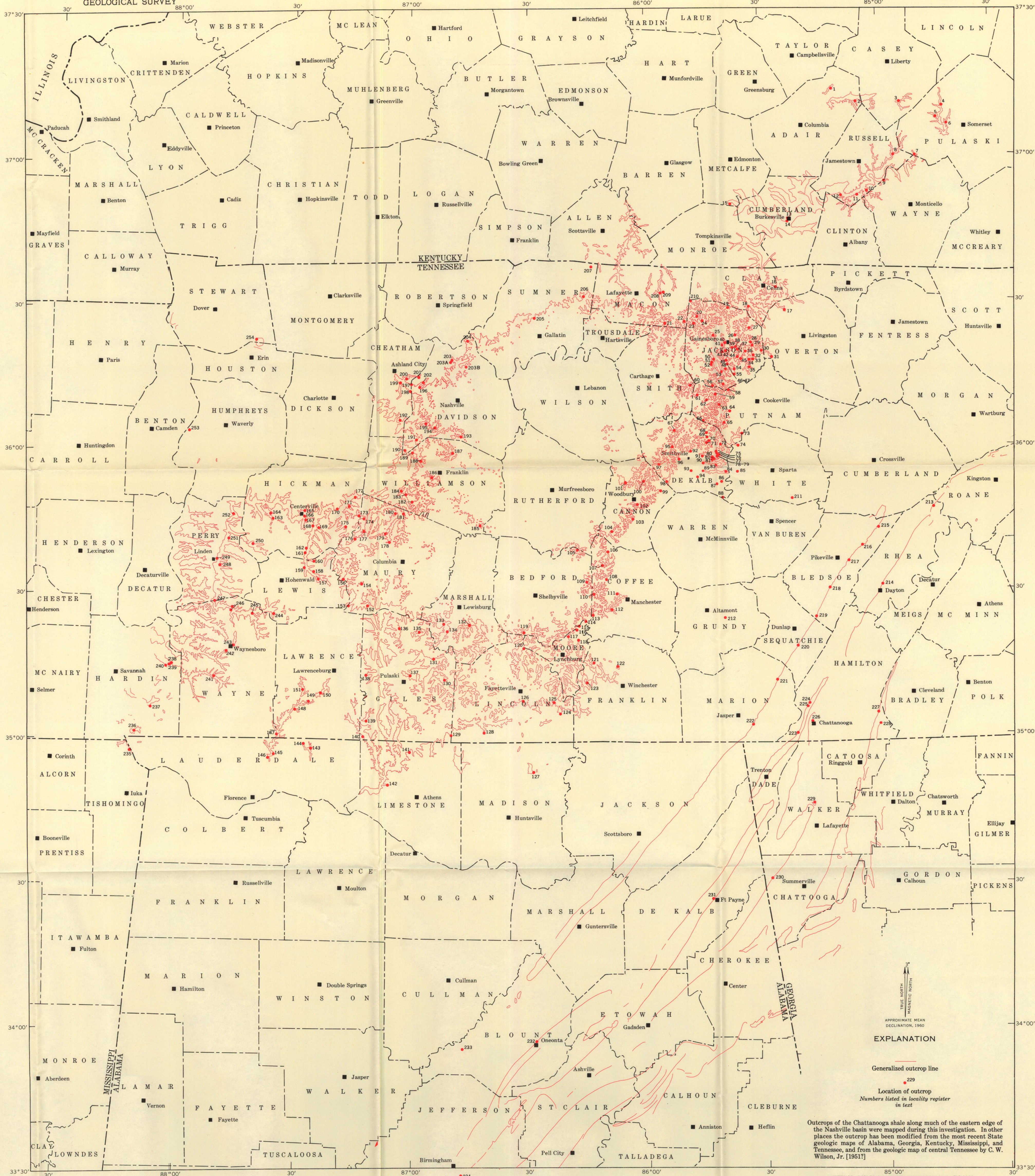
OUTCROPS OF THE CHATTANOOGA SHALE AND MAURY FORMATION IN CENTRAL TENNESSEE AND NEARBY AREAS
