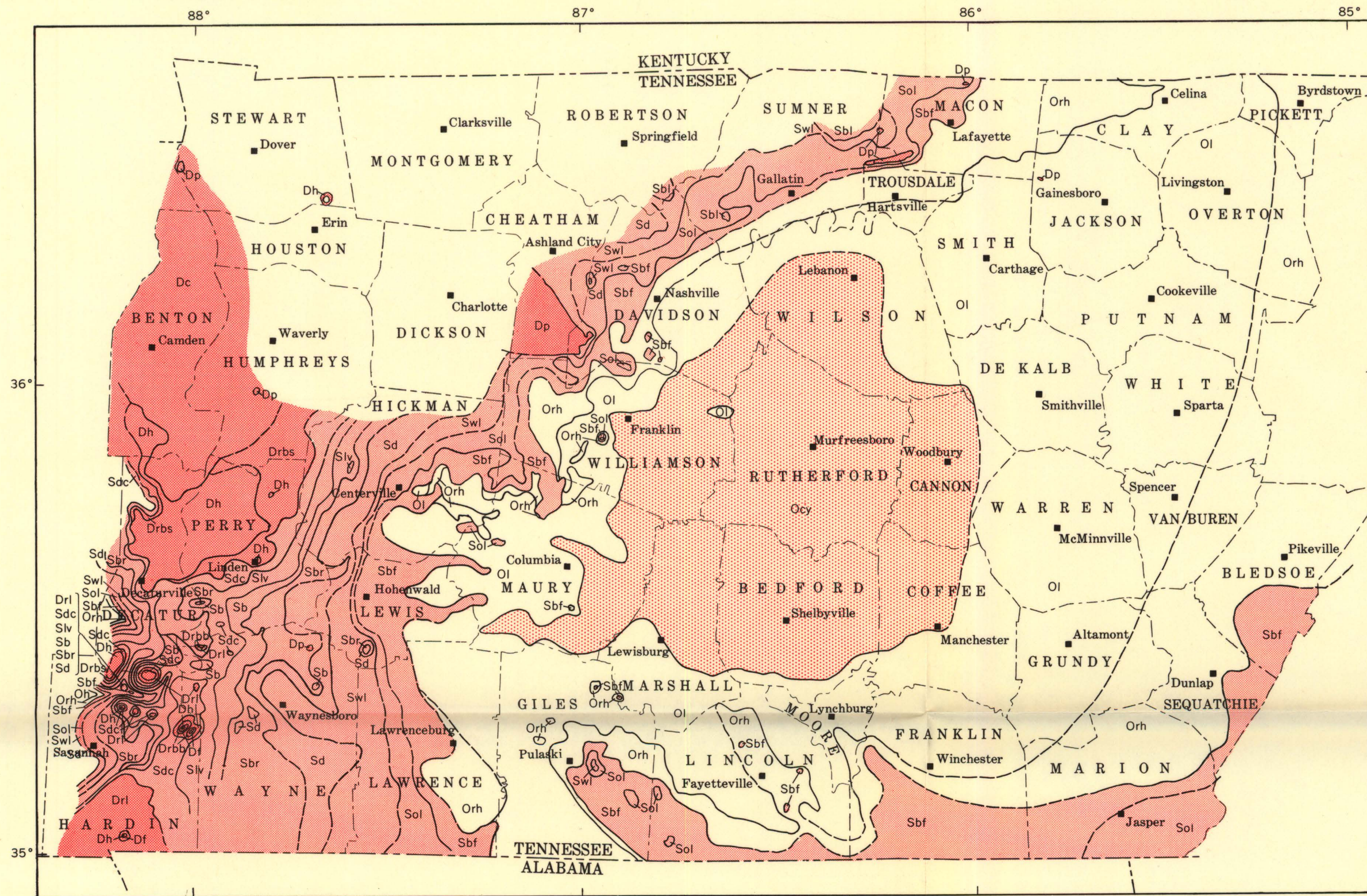
GEOLOGIC MAP OF CENTRAL TENNESSEE JUST PRIOR TO DEPOSITION OF THE CHATTANOOGA SHALE
