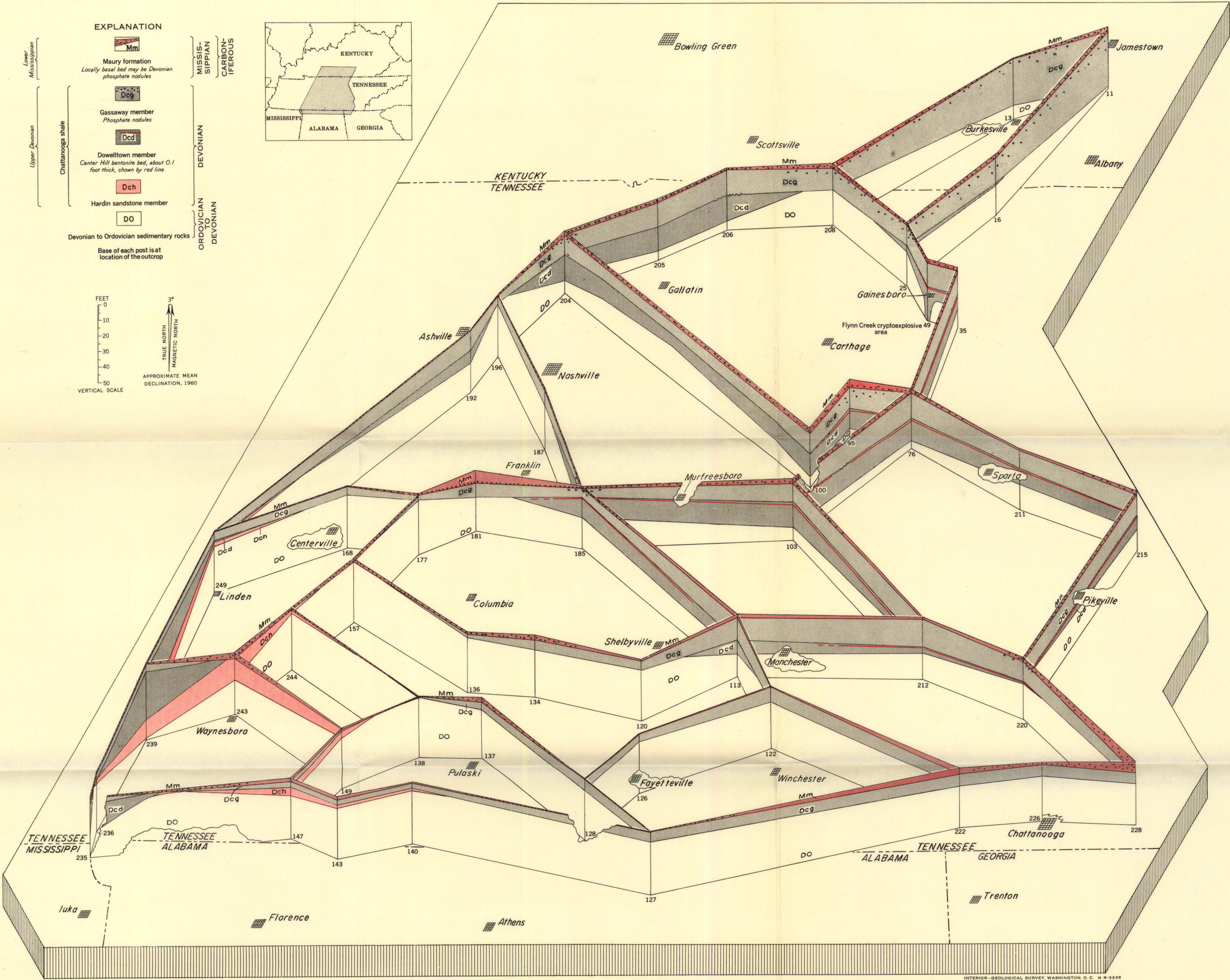
FENCE DIAGRAM SHOWING RELATIONS OF THE SEVERAL UNITS OF THE CHATTANOOGA SHALE AND THE MAURY FORMATION
