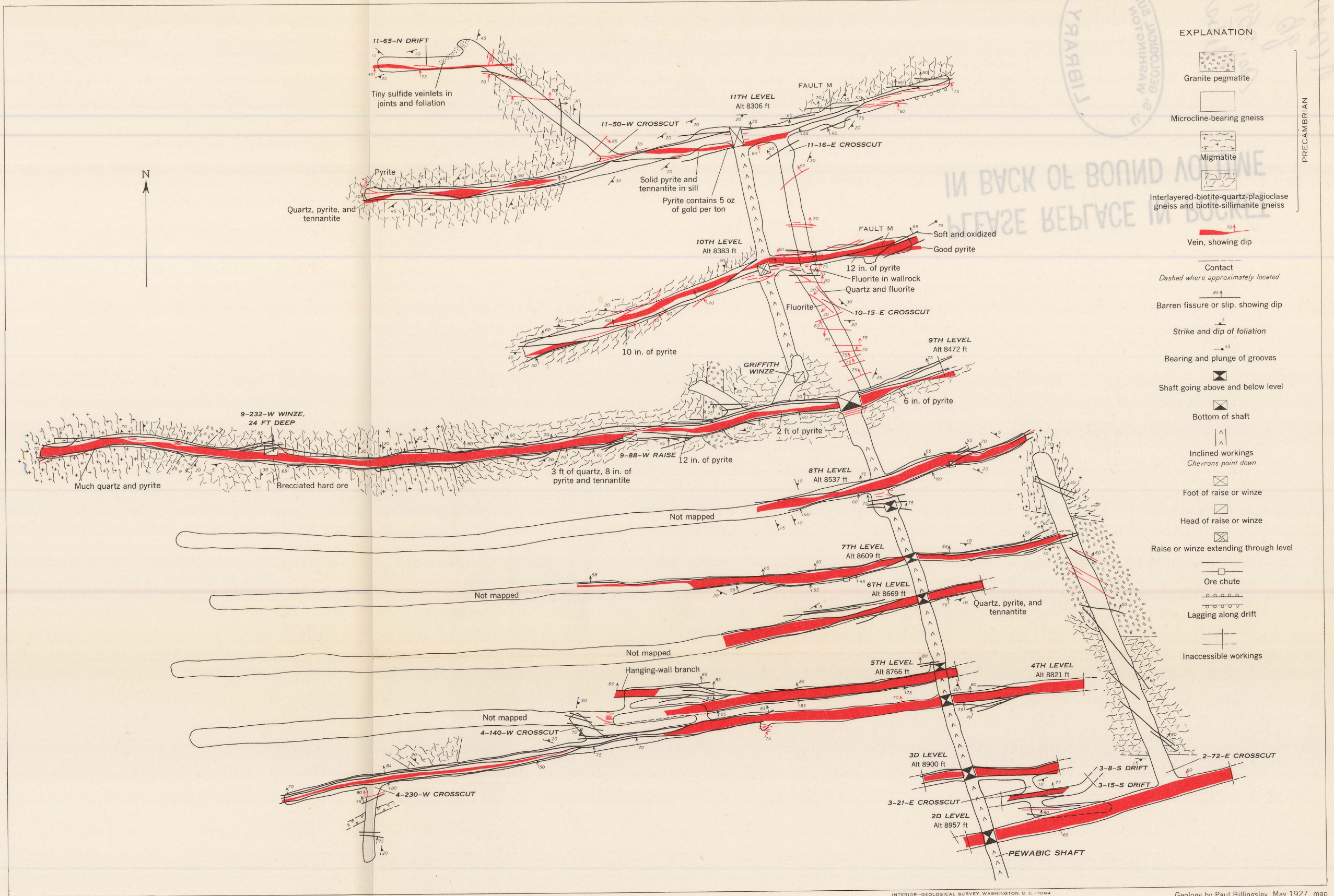
GEOLOGIC MAP OF PART OF THE PEWABIC MINE, CENTRAL CITY DISTRICT, COLORADO
