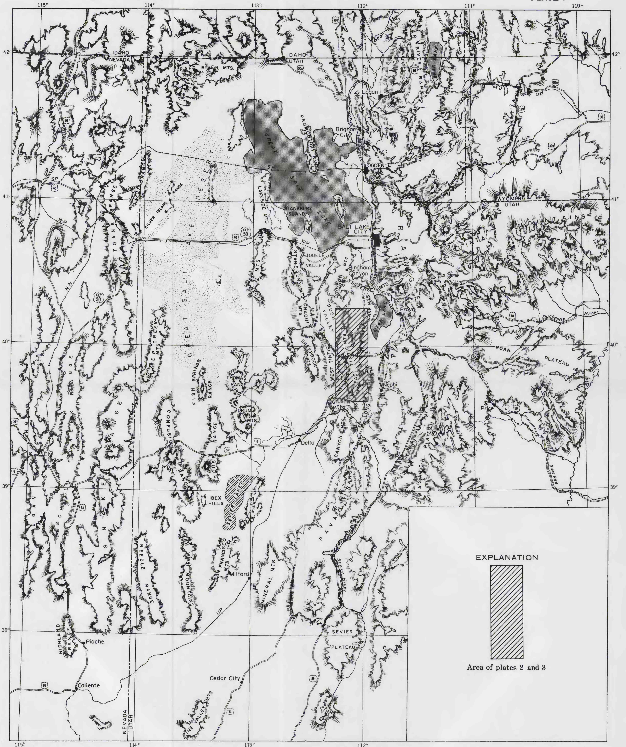
INDEX MAP OF NORTHERN UTAH AND ADJACENT STATES SHOWING LOCATION OF EAST TINTIC MOUNTAINS
