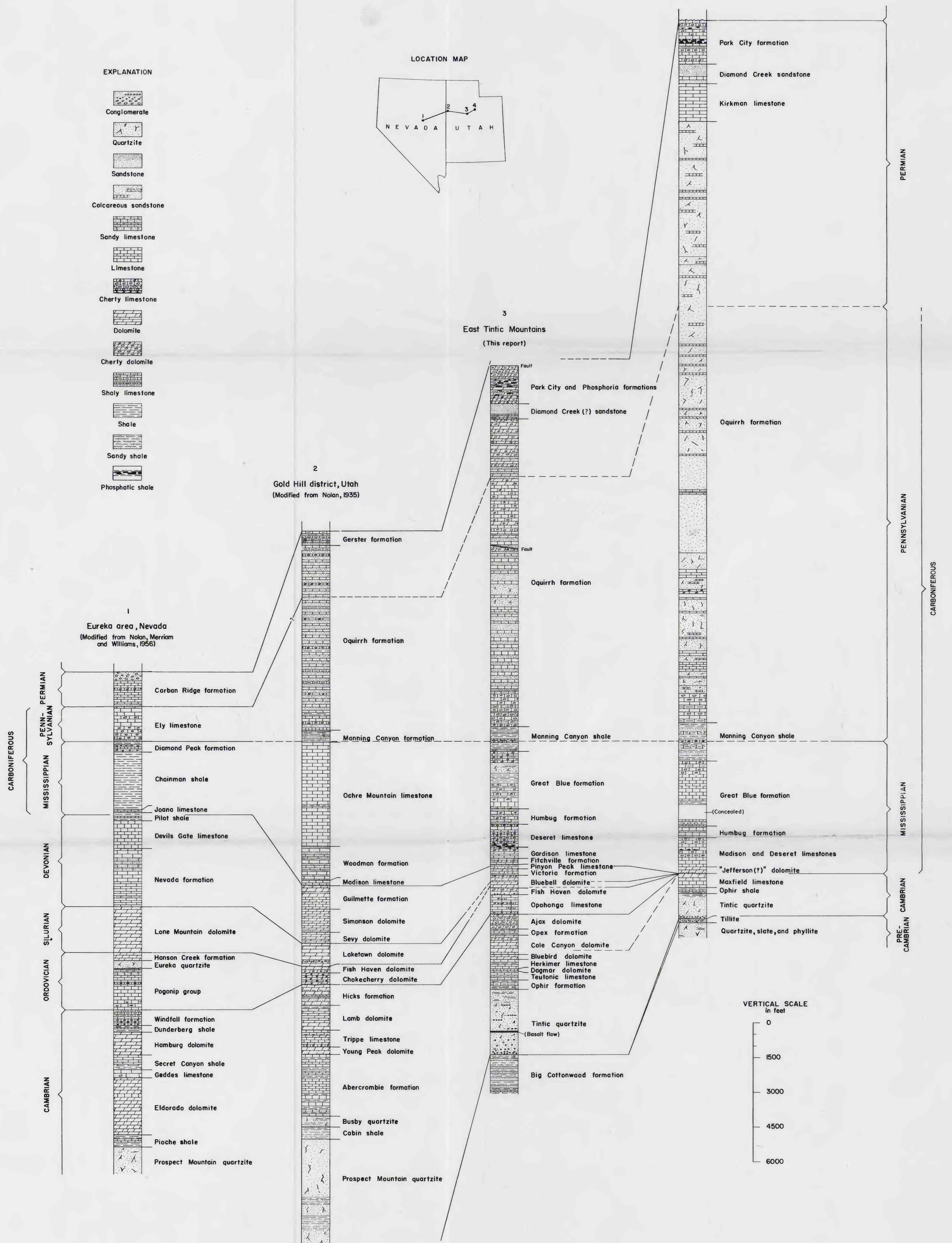
CORRELATION OF SOME PALEOZOIC SECTIONS IN CENTRAL AND WESTERN UTAH, AND EAST-CENTRAL NEVADA
