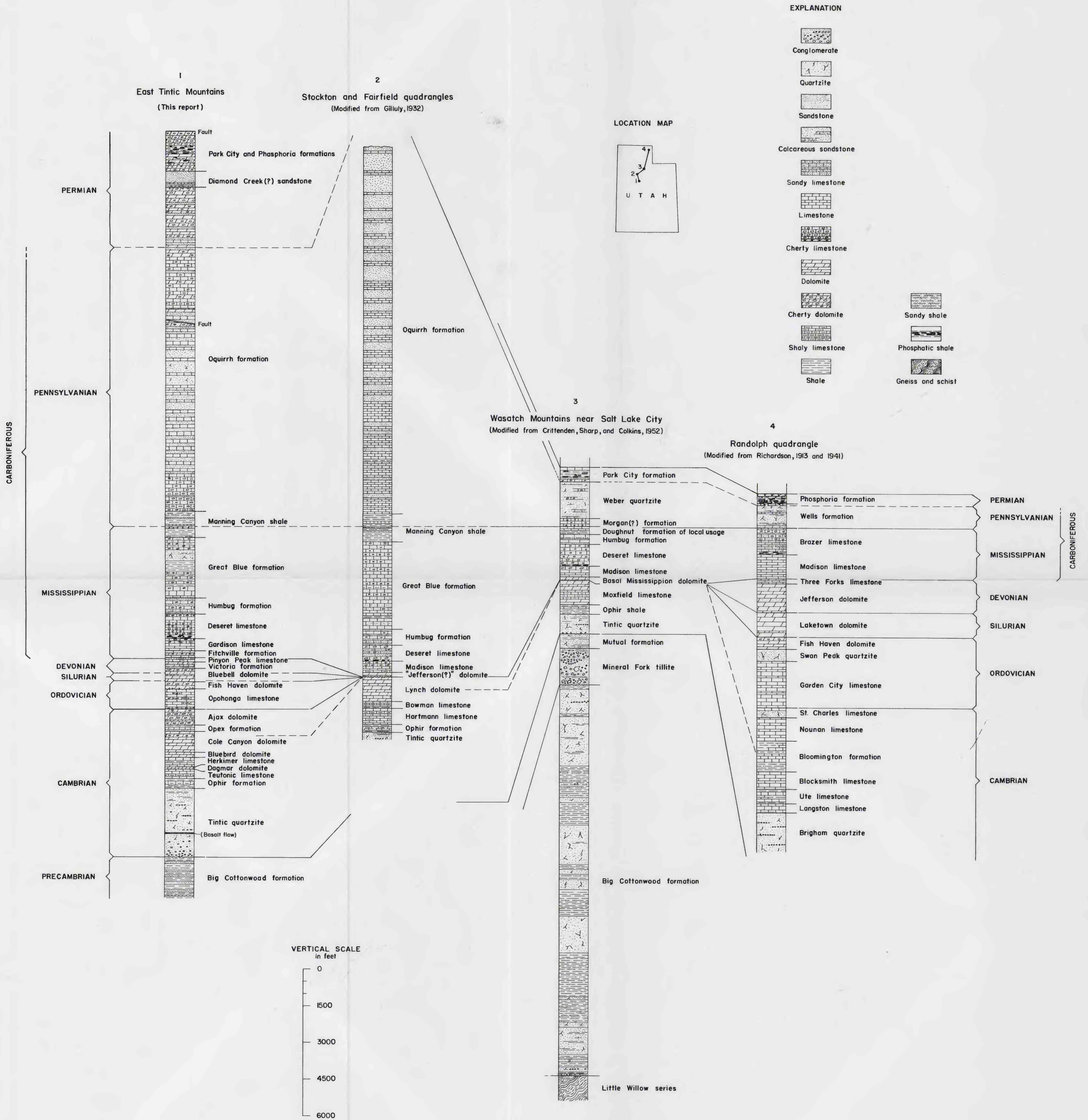
CORRELATION OF SOME PALEOZOIC SECTIONS IN CENTRAL AND NORTHERN UTAH
