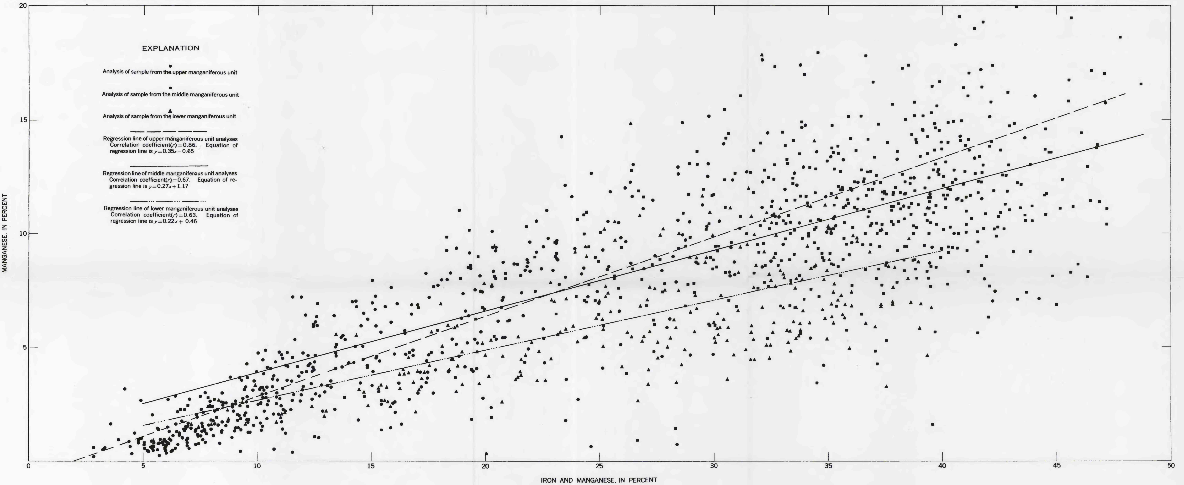
SCATTER DIAGRAM OF THE VARIATION OF Mn WITH RESPECT TO TOTAL Mn AND Fe
