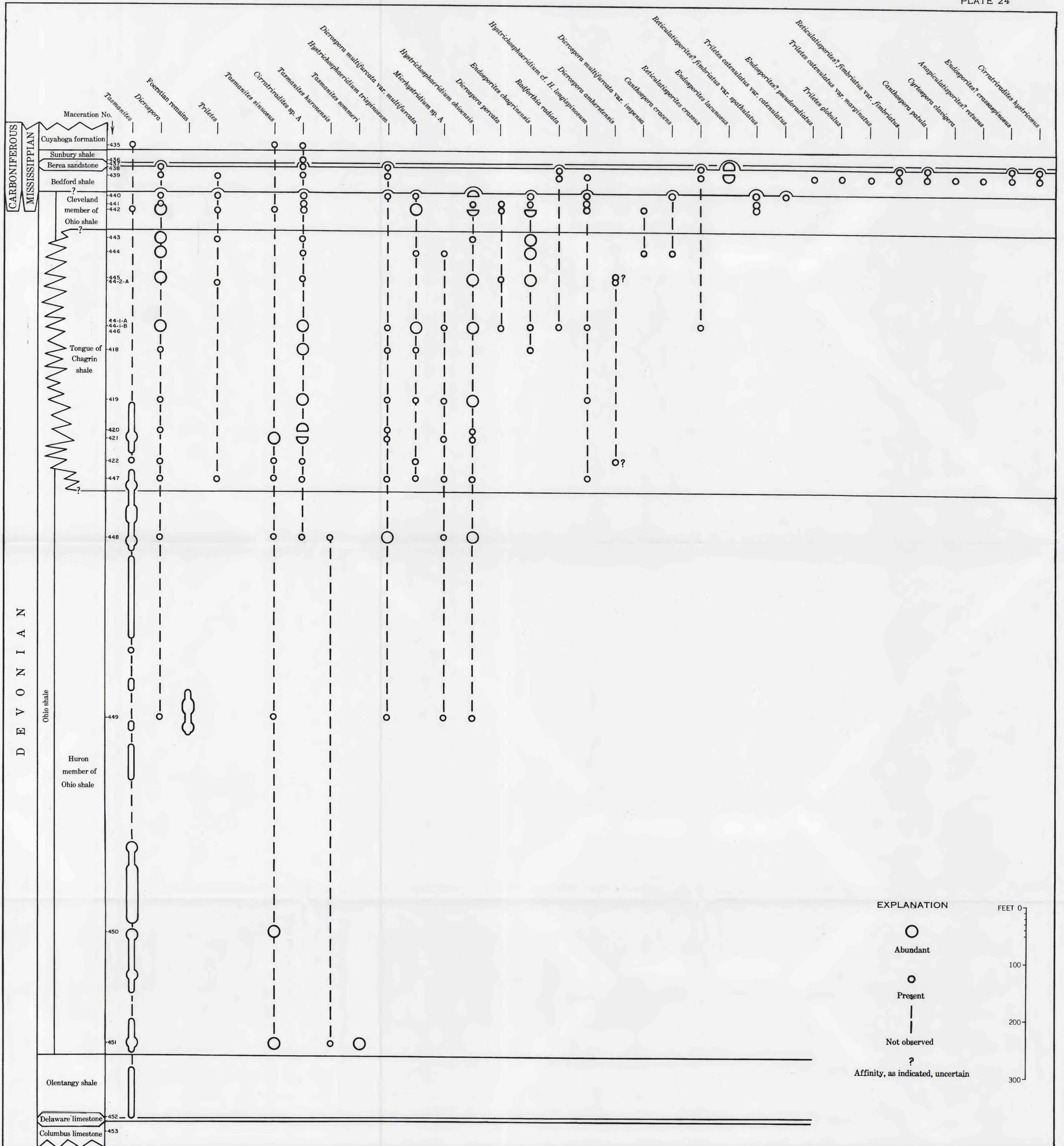
STRATIGRAPHIC OCCURRENCE AND RELATIVE ABUNDANCE OF MICROFOSSILS FROM THE BARBERTON CORE AT LOCALITY 6
