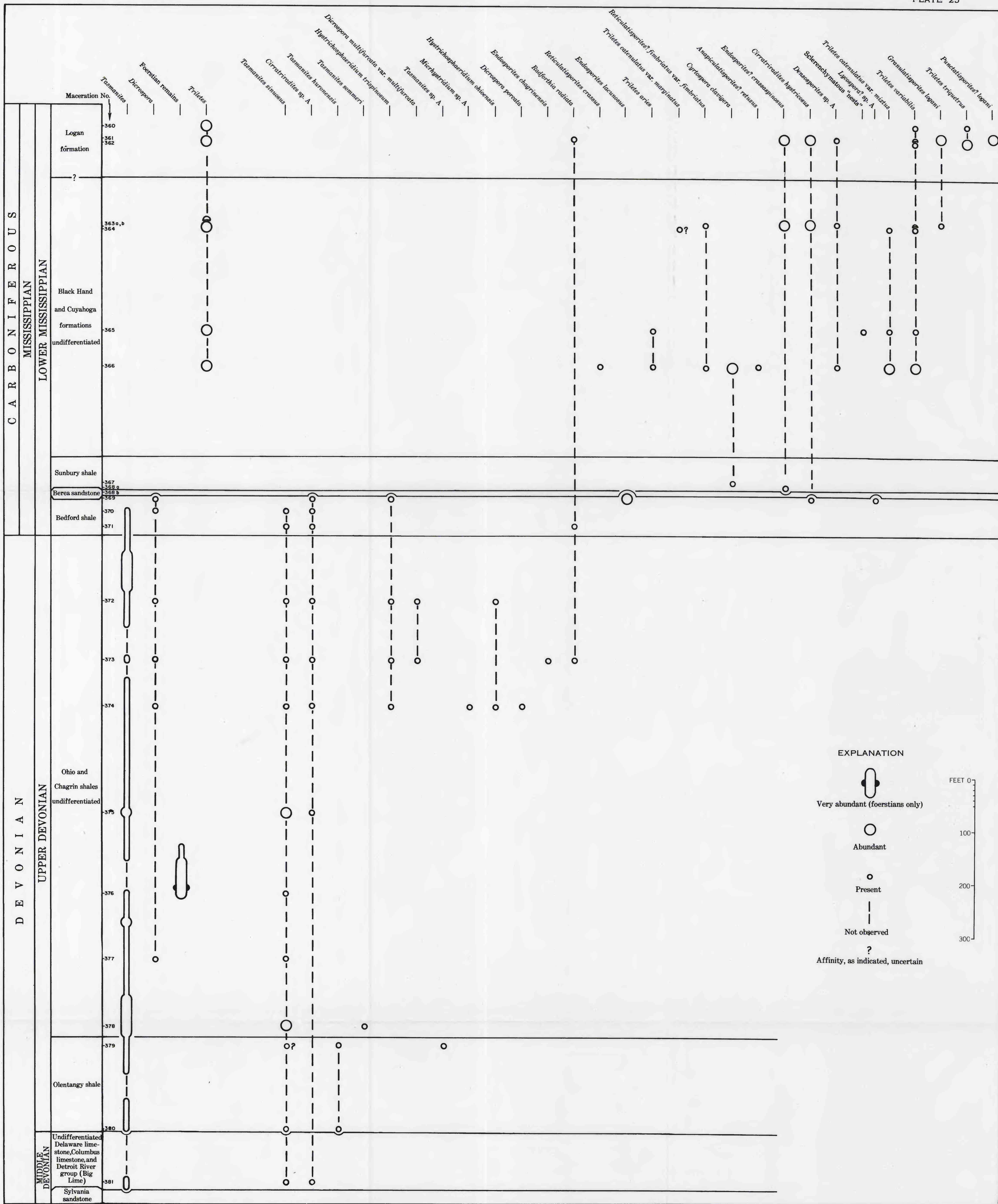
STRATIGRAPHIC OCCURRENCE AND RELATIVE ABUNDANCE OF MICROFOSSILS IN CUTTINGS FROM THE NEWCASTLE WELL AT LOCALITY 7
