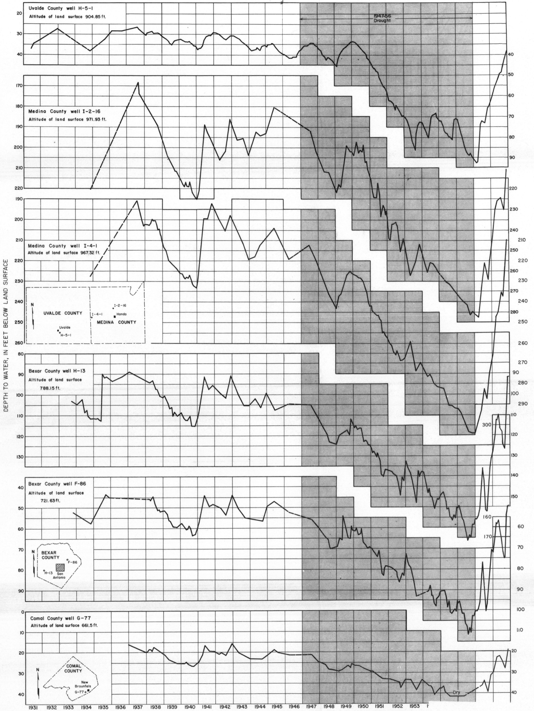
HYDROGRAPHS OF 6 WELLS IN THE BALCONES FAULT-ZONE AQUIFER, 19
