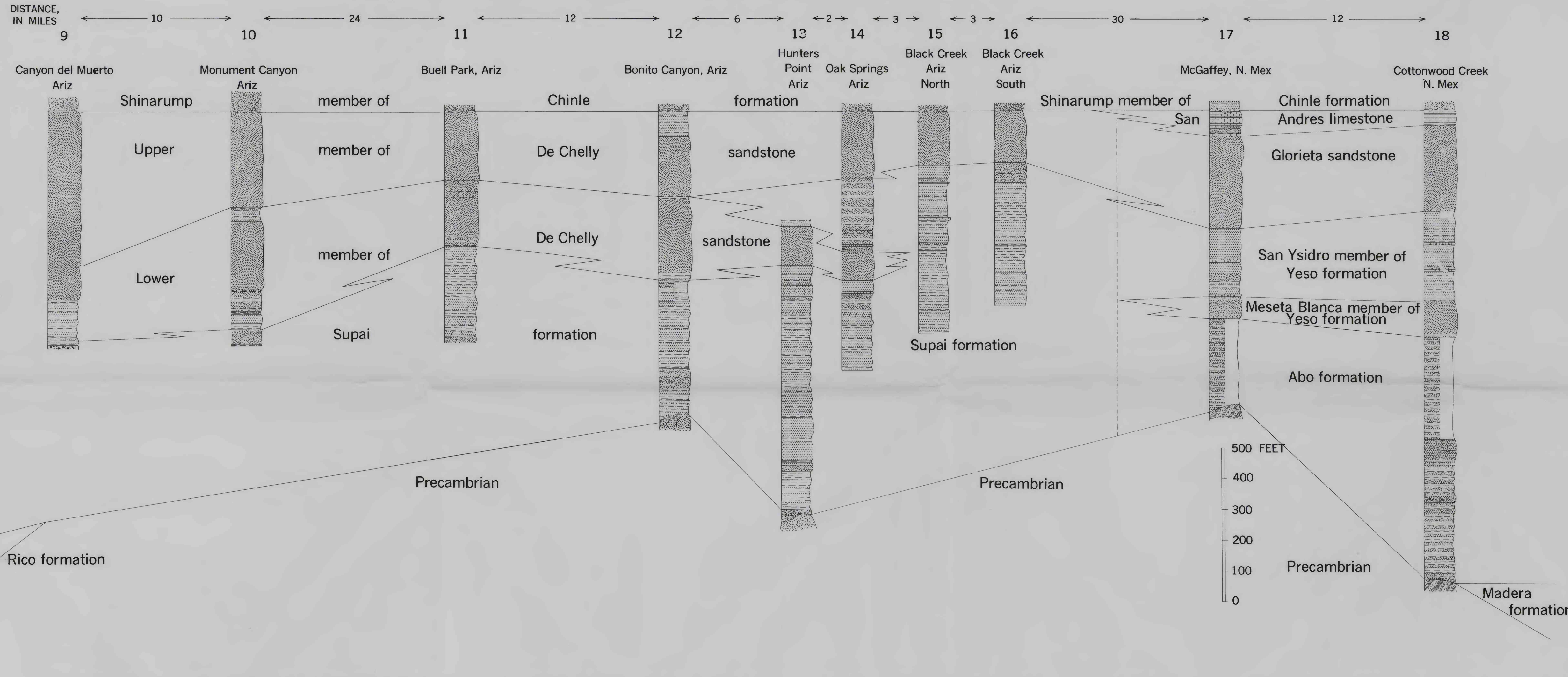
GRAPHIC SECTIONS OF PERMIAN STRATA BETWEEN NOKAI CANYON, UTAH, CANYON DEL MUERTO, ARIZONA, AND COTTONWOOD CREEK, NEW MEXICO
