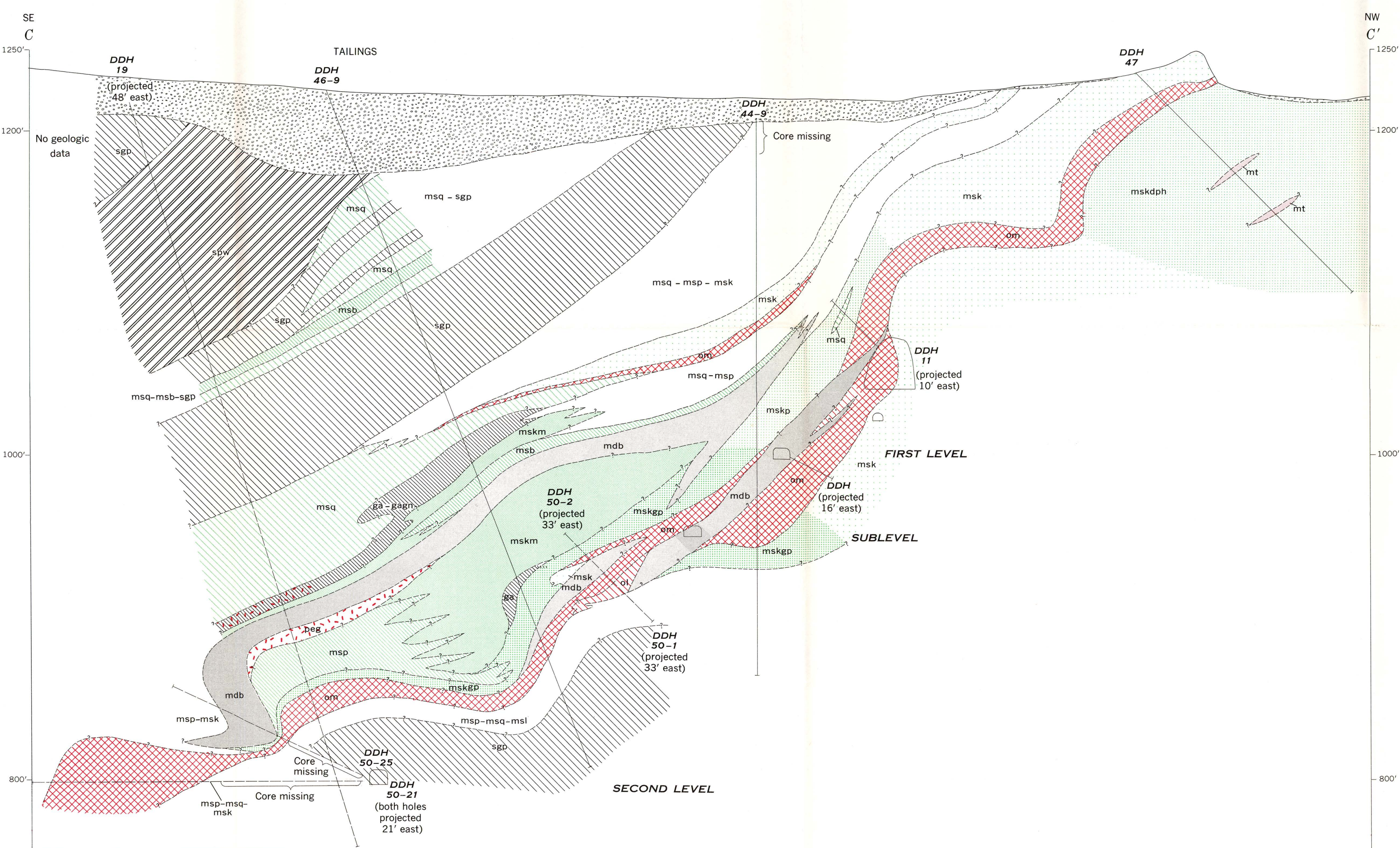
GEOLOGIC SECTIONS ALONG LINES A-A' TO C-C', CLIFTON MINE, ST. LAWRENCE COUNTY, NEW YORK
